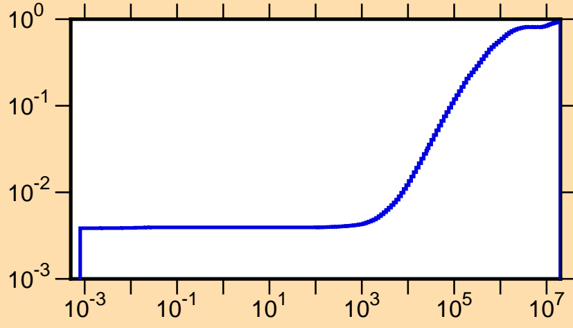
\mu vs. E for ^{175}\text{Lu}(\text{mt251})
