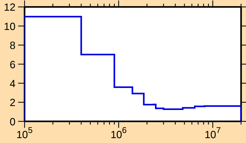
\Delta\sigma/\sigma vs. E for ^{175}\text{Lu}(n,\text{nonel.})
