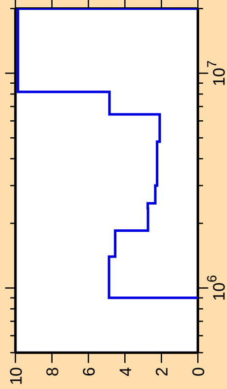
\Delta\sigma/\sigma vs. E for ^{175}\text{Lu}(n,n\text{cont.})
