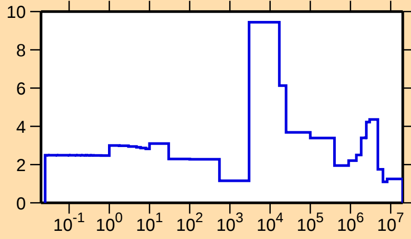
\Delta\sigma/\sigma vs. E for ^{175}\text{Lu}(n,\text{el.})
