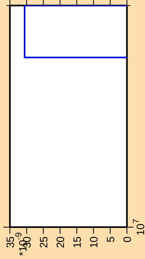
\Delta\sigma/\sigma vs. E for ^{176}\text{Lu} (mt 42)
