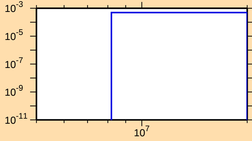
\sigma vs. E for ^{176}\text{Lu}(n,np)
