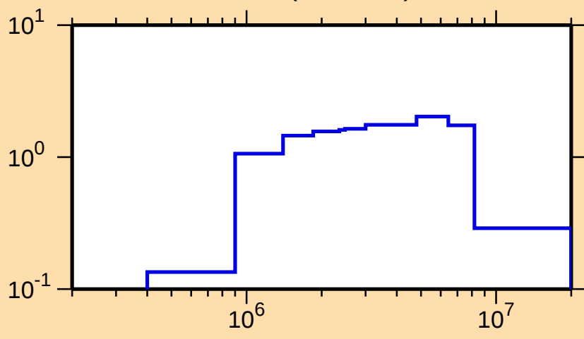
\sigma vs. E for ^{176}\text{Lu}(n,n\text{cont.})
