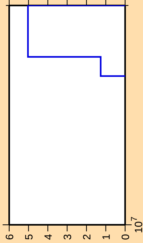
\Delta\sigma/\sigma vs. E for ^{176}\text{Lu}(n,p\alpha)
