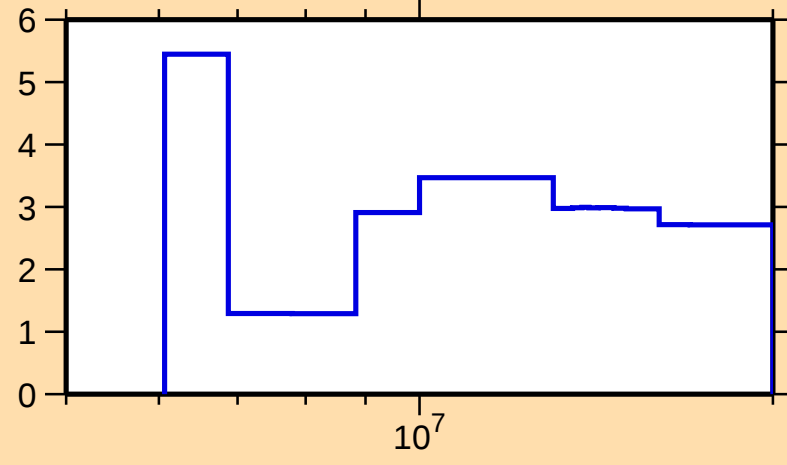
\Delta\sigma/\sigma vs. E for ^{176}\text{Lu}(n,\text{tot.})
