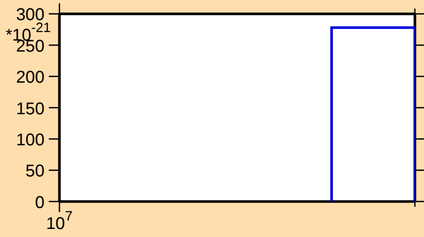
\sigma vs. E for ^{176}\text{Lu} (mt 42)
