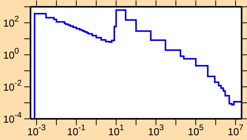
\sigma vs. E for ^{176}\text{Lu}(n,\gamma)
