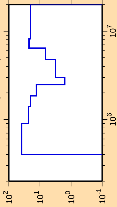
\Delta\sigma/\sigma vs. E for ^{176}\text{Lu}(n,\text{ncont.})
