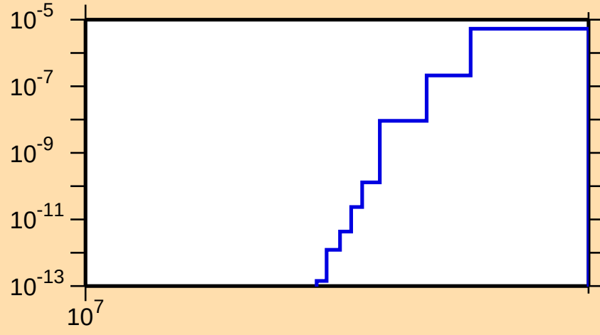
\sigma vs. E for ^{177}\text{Lu}(n,\text{nd})
