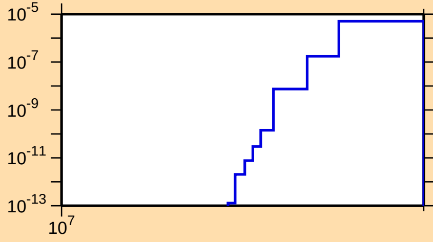
\sigma vs. E for ^{177}\text{Lu}(n,nt)
