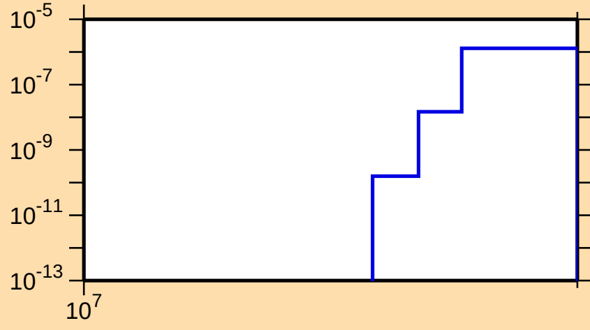
\sigma vs. E for ^{177}\text{Lu}(n,2np)
