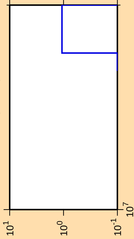
\Delta\sigma/\sigma vs. E for ^{177}\text{Lu}(n,3n\alpha)
