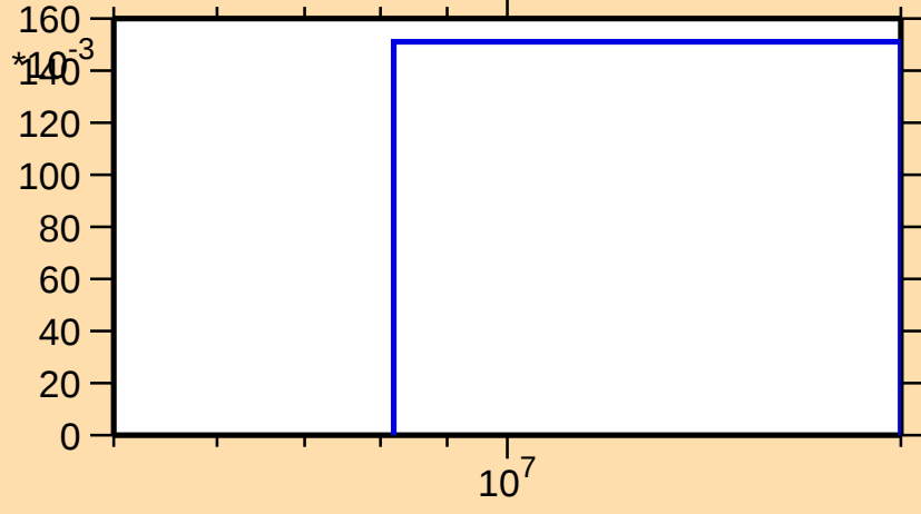
\sigma vs. E for ^{177}\text{Lu}(n,3n)
