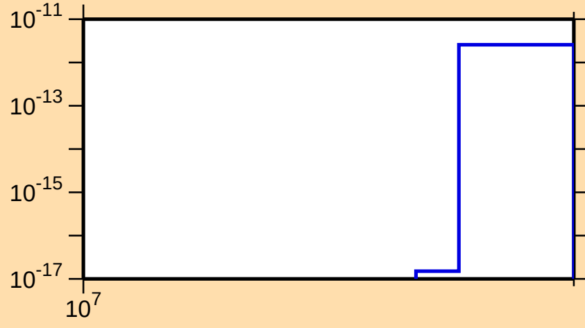
\sigma vs. E for ^{177}\text{Lu}(n,3n\alpha)
