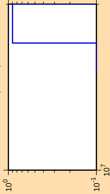
\Delta\sigma/\sigma vs. E for ^{177}\text{Lu} (mt 11)
