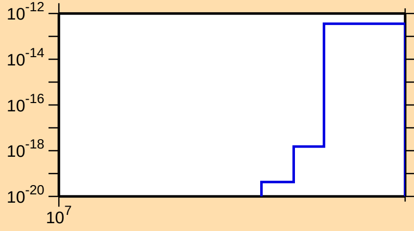
\sigma vs. E for ^{177}\text{Lu} (mt 11)
