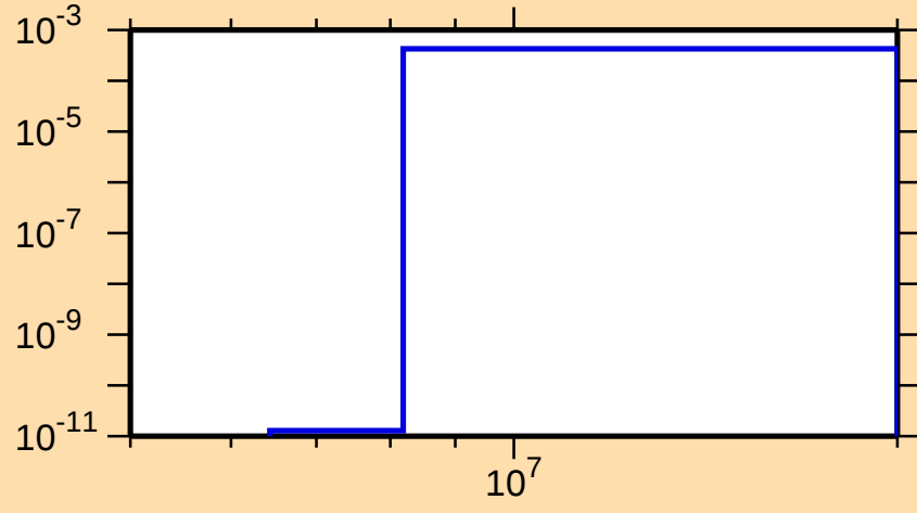
\sigma vs. E for ^{177}\text{Lu}(n,d)
