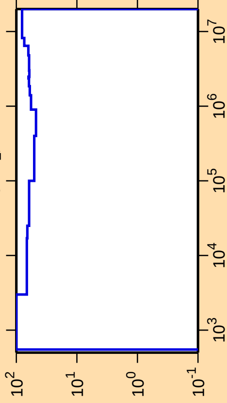
\Delta\sigma/\sigma vs. E for ^{177}\text{Lu}(n,n_1)
