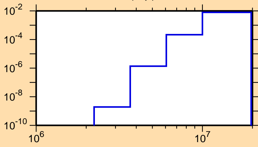
\sigma vs. E for ^{178}\text{Lu}(n,p)
