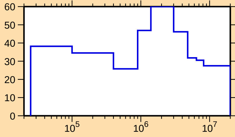
\Delta\sigma/\sigma vs. E for ^{178}\text{Lu}(n,n_1)
