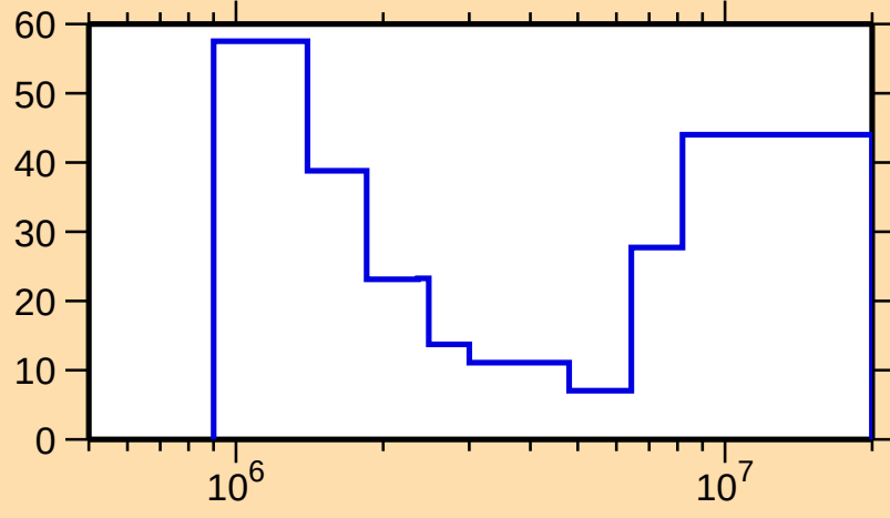
\Delta\sigma/\sigma vs. E for ^{178}\text{Lu}(n,n\text{cont.})
