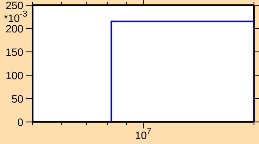
\sigma vs. E for ^{178}\text{Lu}(n,3n)
