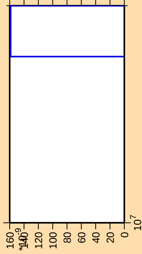
\Delta\sigma/\sigma vs. E for ^{178}\text{Lu} (mt 42)
