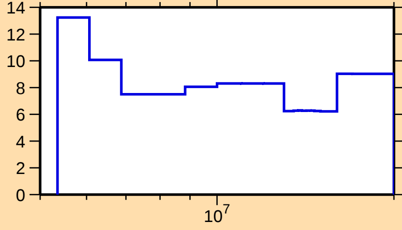
\Delta\sigma/\sigma vs. E for ^{178}\text{Lu}(n,\text{el.})
