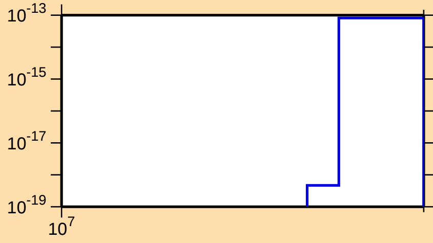
\sigma vs. E for ^{178}\text{Lu}(n,3n\alpha)
