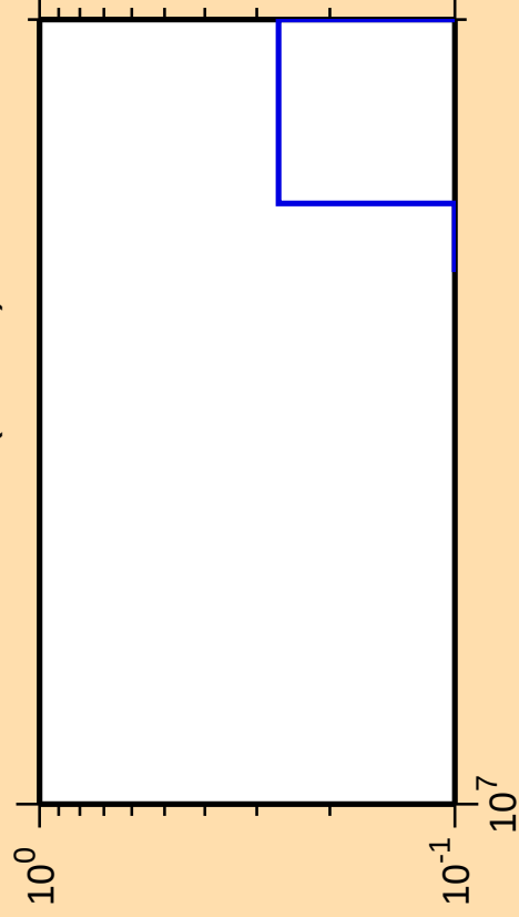
\Delta\sigma/\sigma vs. E for ^{178}\text{Lu}(n,3n\alpha)
