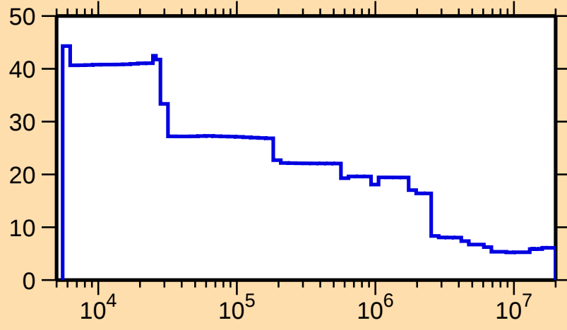
\Delta\sigma/\sigma vs. E for ^{178}\text{Lu}(n,\text{nonel.})
