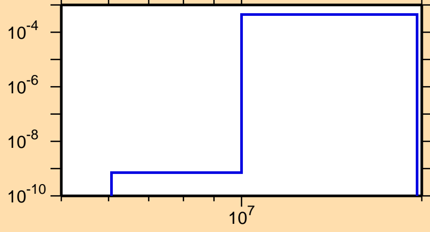
\sigma vs. E for ^{178}\text{Lu}(n,d)
