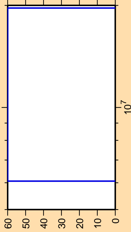
\Delta\sigma/\sigma vs. E for ^{178}\text{Lu}(n,d)
