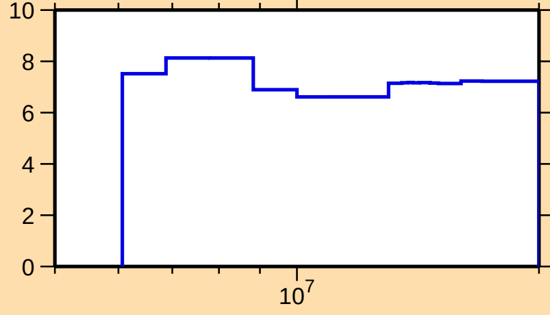
\Delta\sigma/\sigma vs. E for ^{179}\text{Lu}(n,\text{nonel.})
