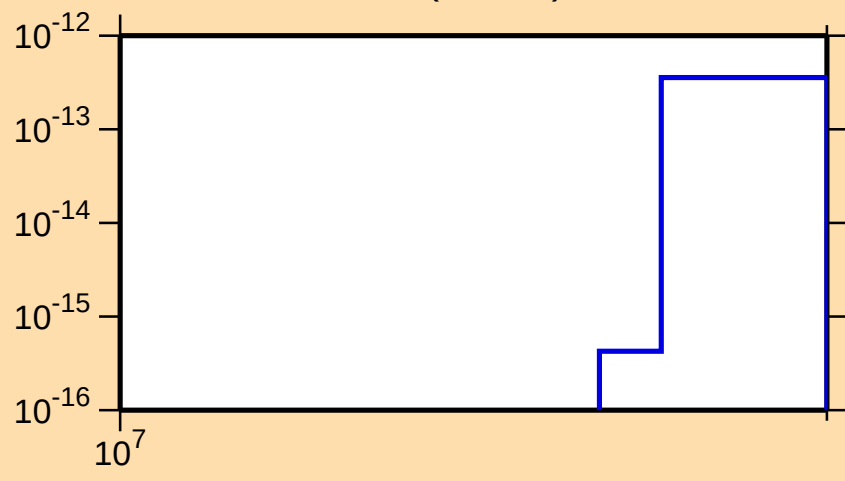
\sigma vs. E for ^{179}\text{Lu}(n,\text{He3})
