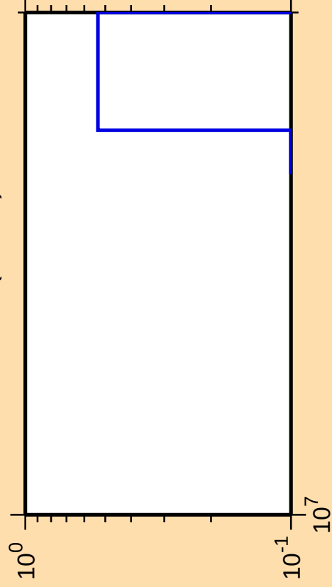
\Delta\sigma/\sigma vs. E for ^{179}\text{Lu}(n,3n\alpha)
