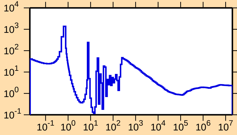
\sigma vs. E for ^{179}\text{Lu}(n,\text{nonel.})
