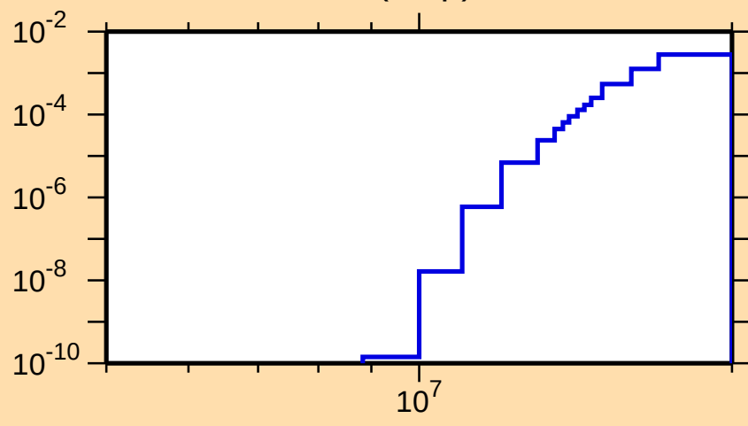
\sigma vs. E for ^{179}\text{Lu}(n,np)
