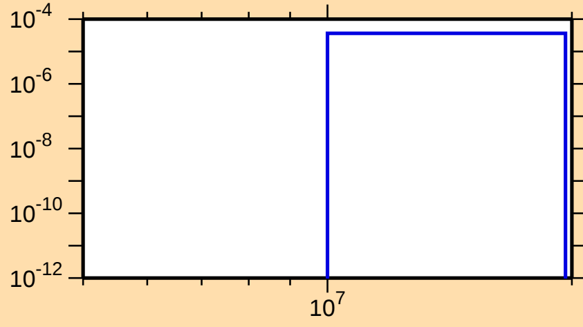
\sigma vs. E for ^{179}\text{Lu}(n,t)
