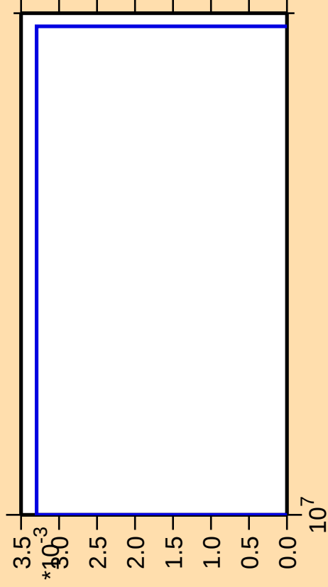
\Delta\sigma/\sigma vs. E for ^{179}\text{Lu}(n,3n\alpha)
