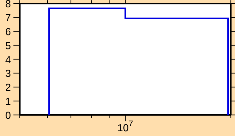
\Delta\sigma/\sigma vs. E for ^{179}\text{Lu}(n,\text{nonel.})
