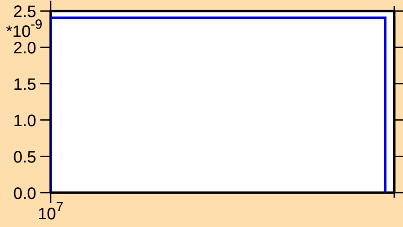
\sigma vs. E for ^{179}\text{Lu}(n,2n\alpha)
