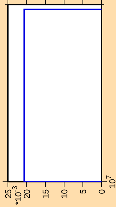
\Delta\sigma/\sigma vs. E for ^{179}\text{Lu}(n,\text{He}3)
