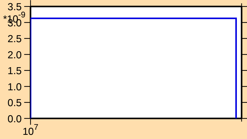
\sigma vs. E for ^{179}\text{Lu}(n,2np)
