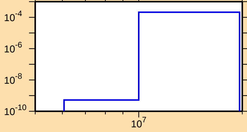
\sigma vs. E for ^{179}\text{Lu}(n,d)
