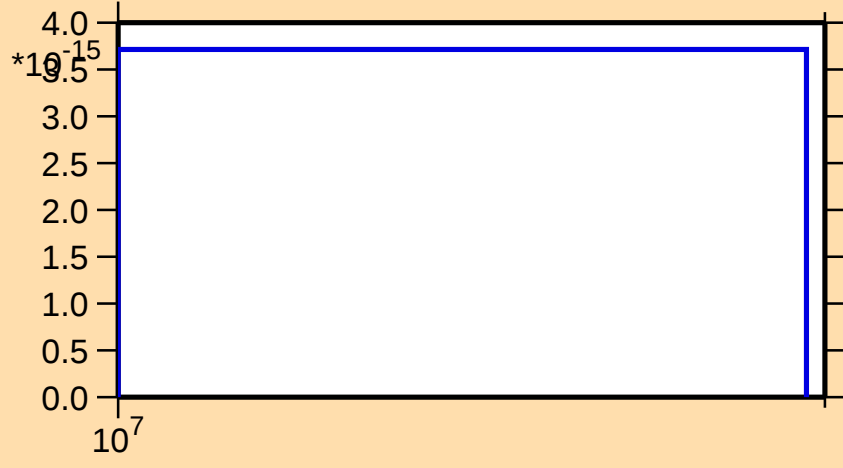
\sigma vs. E for ^{179}\text{Lu}(n,3n\alpha)
