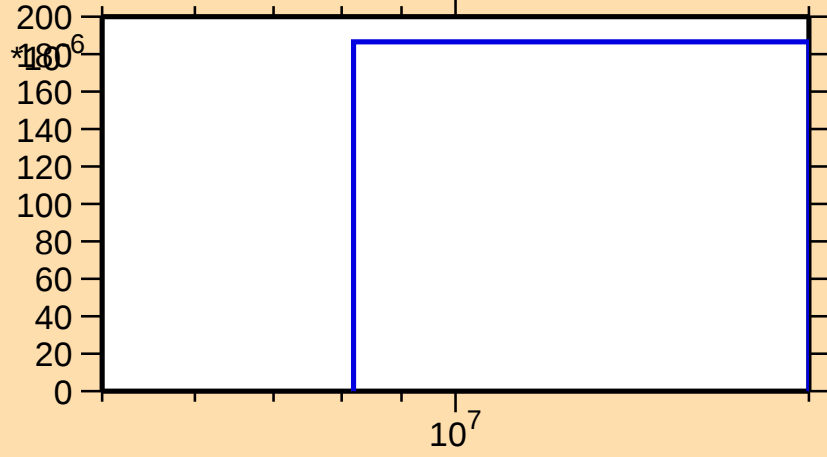
\sigma vs. E for ^{179}\text{Lu}(n,np)
