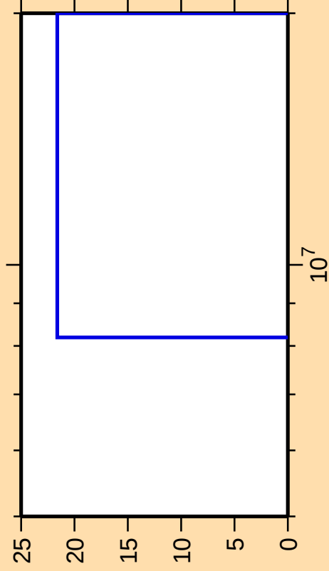
\Delta\sigma/\sigma vs. E for ^{179}\text{Lu}(n,3n)
