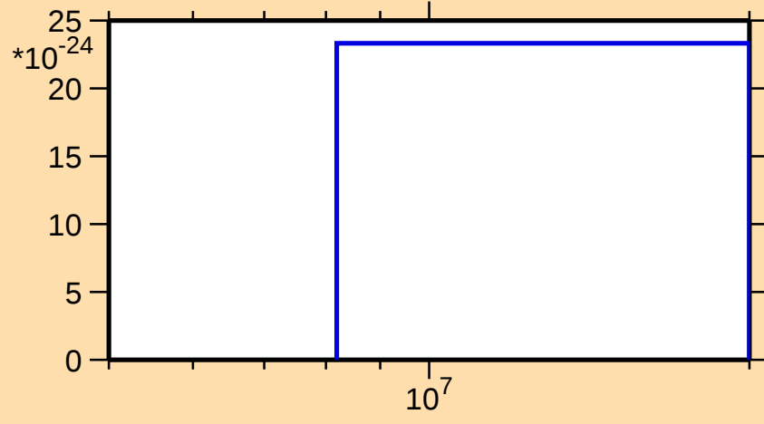
\sigma vs. E for ^{179}\text{Lu} (mt 42)
