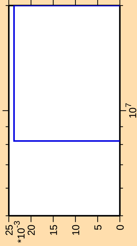
\Delta\sigma/\sigma vs. E for ^{179}\text{Lu}(n,\text{He}3)
