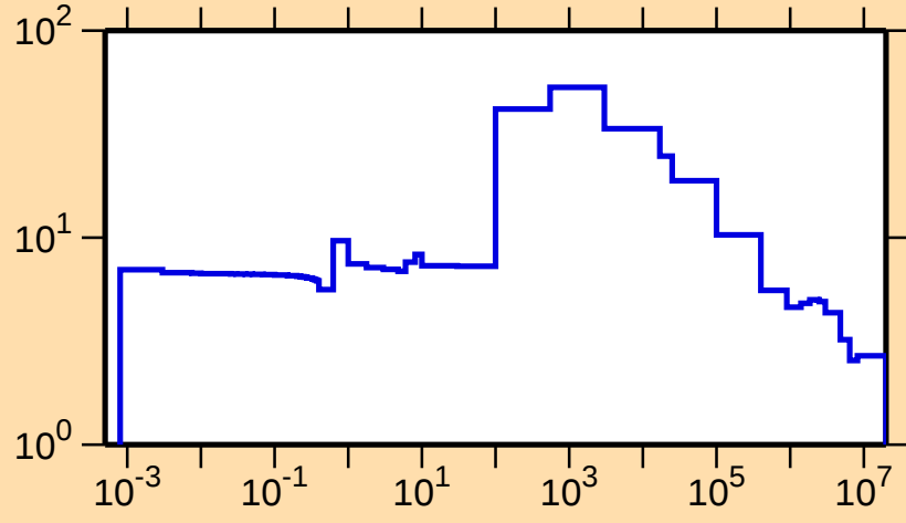
\sigma vs. E for ^{179}\text{Lu}(n,\text{el.})
