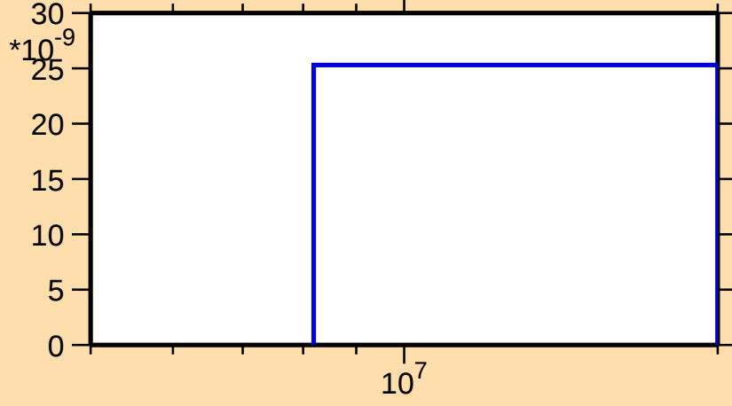
\sigma vs. E for ^{179}\text{Lu}(n,\text{nd})
