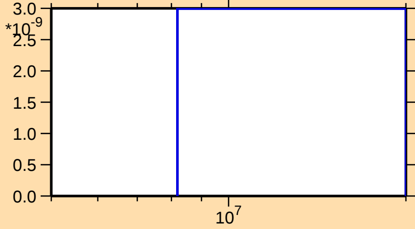
\sigma vs. E for ^{179}\text{Lu}(n,2np)
