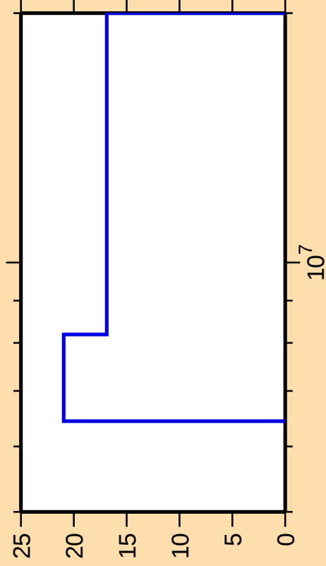
\Delta\sigma/\sigma vs. E for ^{179}\text{Lu}(n,2n)
