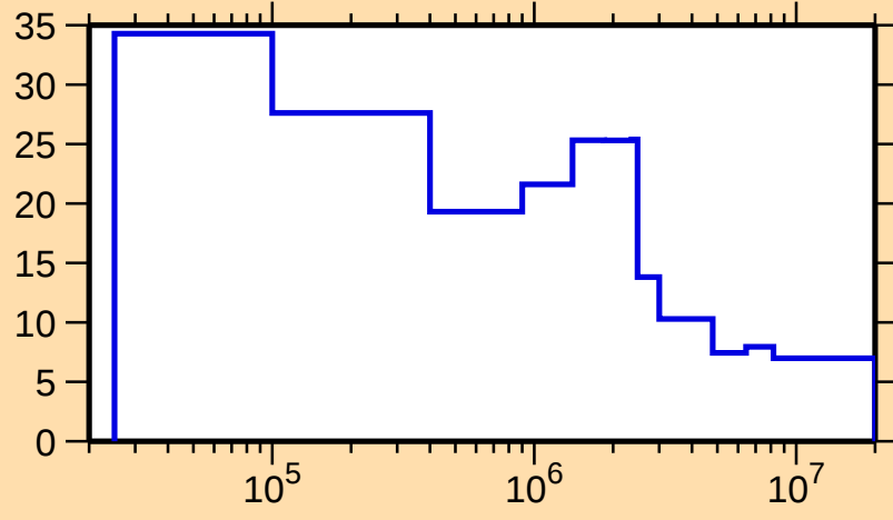
\Delta\sigma/\sigma vs. E for ^{179}\text{Lu}(n,\text{nonel.})
