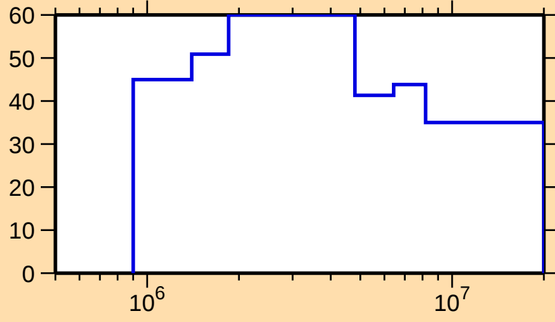
\Delta\sigma/\sigma vs. E for ^{179}\text{Lu}(n,n_1)
