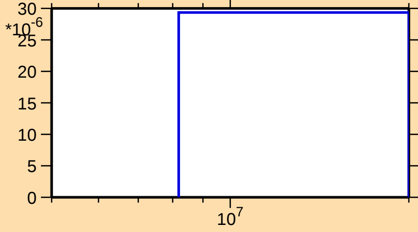
\sigma vs. E for ^{179}\text{Lu}(n,t)
