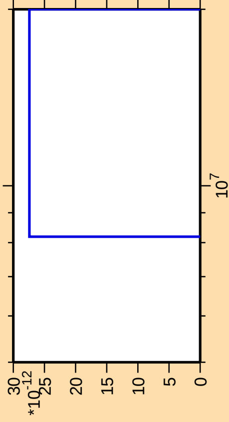
\Delta\sigma/\sigma vs. E for ^{179}\text{Lu} (mt 42)
