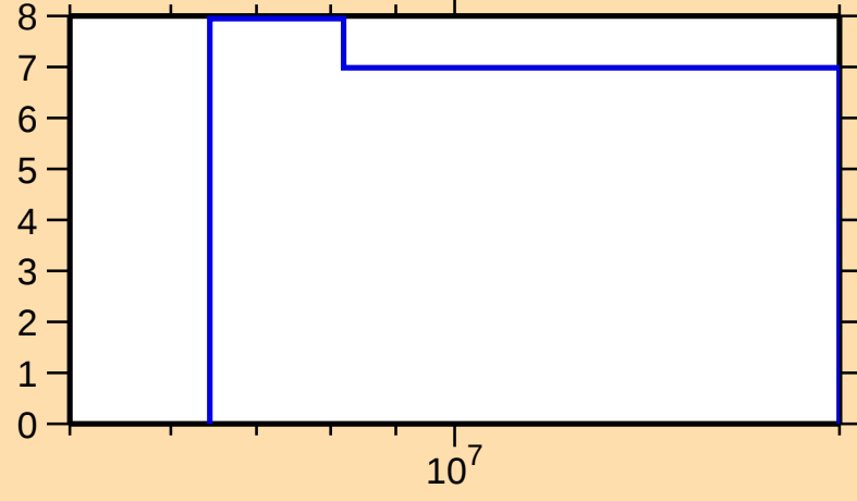
\Delta\sigma/\sigma vs. E for ^{179}\text{Lu}(n,\text{nonel.})
