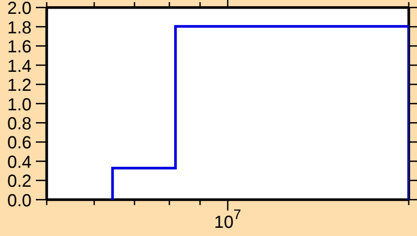
\sigma vs. E for ^{179}\text{Lu}(n,2n)
