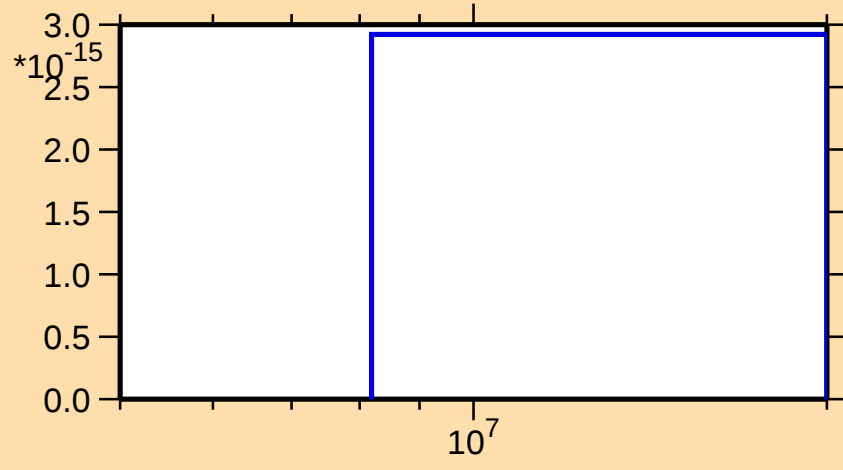
\sigma vs. E for ^{179}\text{Lu}(n,\text{He}3)
