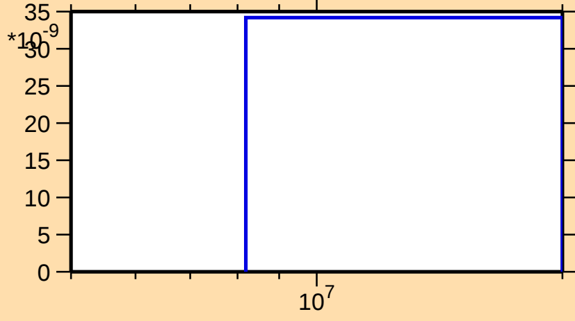
\sigma vs. E for ^{179}\text{Lu}(n,nt)
