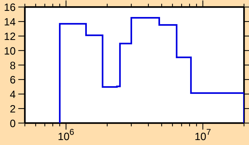
\Delta\sigma/\sigma vs. E for ^{179}\text{Lu}(n,\text{tot.})
