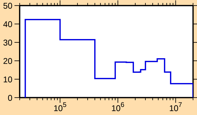
\Delta\sigma/\sigma vs. E for ^{179}\text{Lu}(n,\text{el.})
