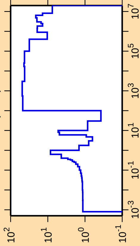
\Delta\sigma/\sigma vs. E for ^{179}\text{Lu}(n,\text{el.})
