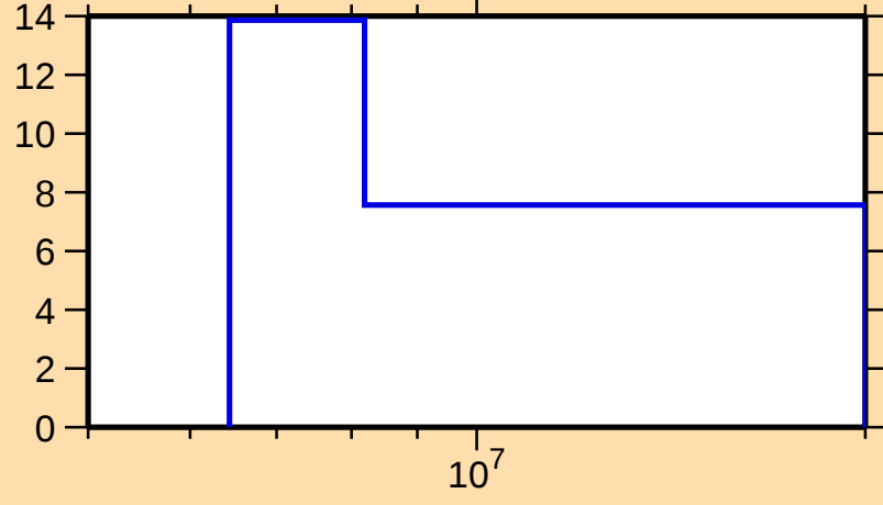
\Delta\sigma/\sigma vs. E for ^{179}\text{Lu}(n,\text{el.})
