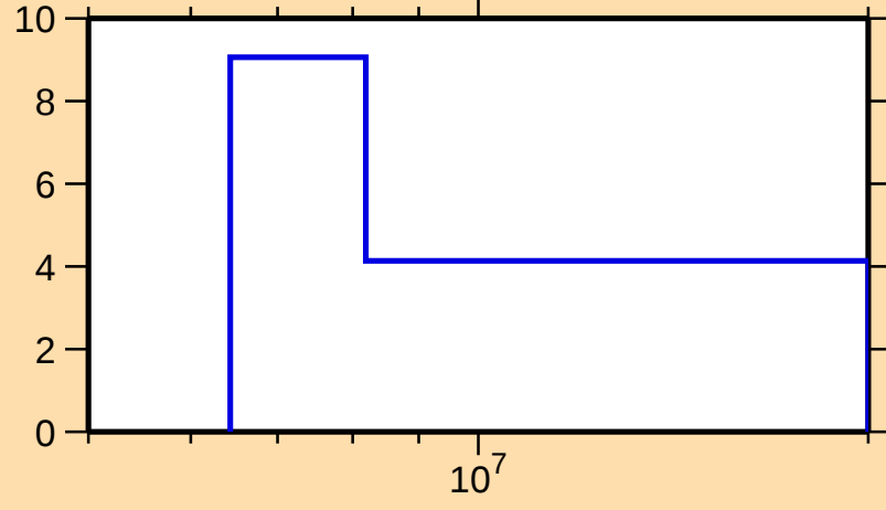
\Delta\sigma/\sigma vs. E for ^{179}\text{Lu}(n,\text{tot.})
