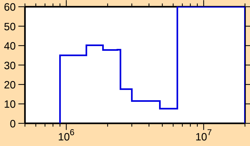
\Delta\sigma/\sigma vs. E for ^{179}\text{Lu}(n,\text{inel.})
