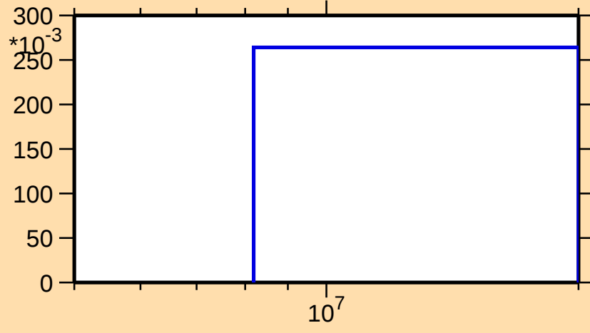
\sigma vs. E for ^{179}\text{Lu}(n,3n)
