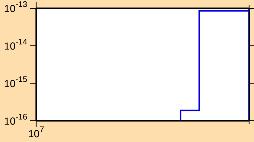
\sigma vs. E for ^{181}\text{Lu} (mt 11)
