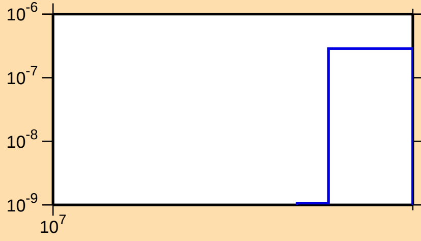
\sigma vs. E for ^{181}\text{Lu}(n,2np)
