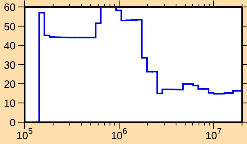
\Delta\sigma/\sigma vs. E for ^{181}\text{Lu}(n,n_1)
