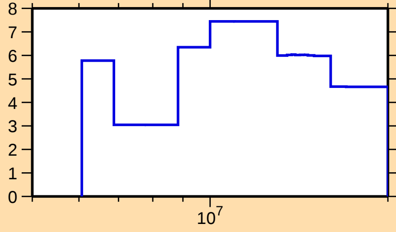
\Delta\sigma/\sigma vs. E for ^{181}\text{Lu}(n,\text{el.})
