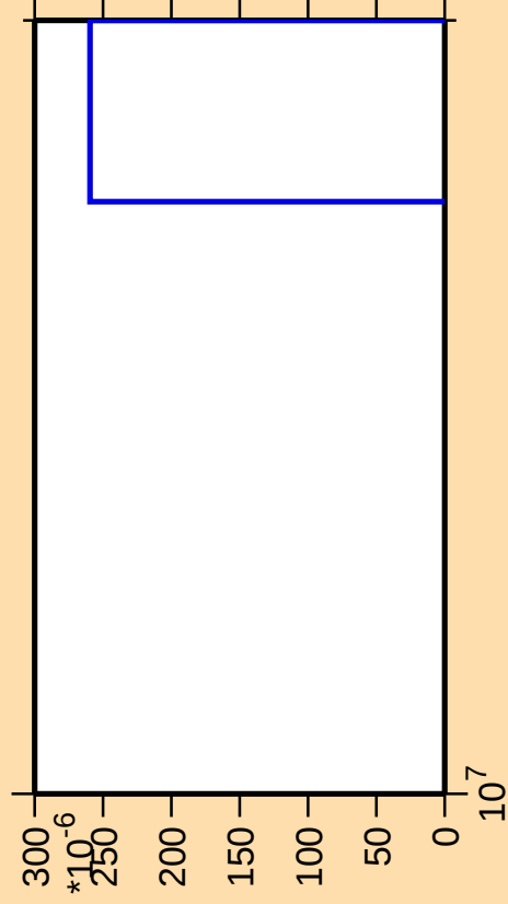
\Delta\sigma/\sigma vs. E for ^{181}\text{Lu} (mt 42)
