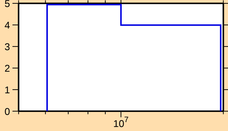
\Delta\sigma/\sigma vs. E for ^{181}\text{Lu}(n,\text{nonel.})
