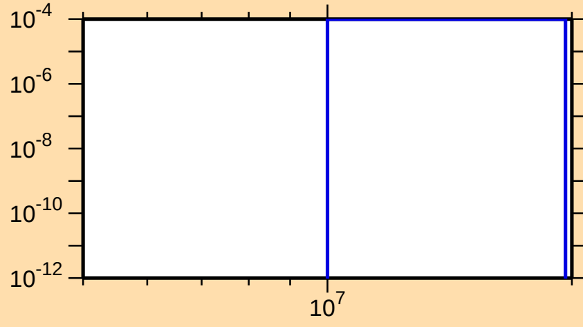
\sigma vs. E for ^{181}\text{Lu}(n,np)
