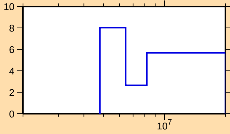
\Delta\sigma/\sigma vs. E for ^{181}\text{Lu}(n,\text{el.})
