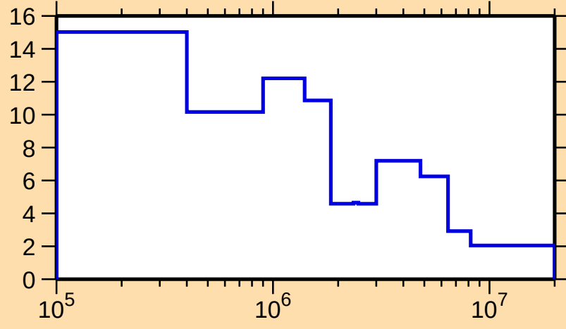
\Delta\sigma/\sigma vs. E for ^{181}\text{Lu}(n,\text{tot.})
