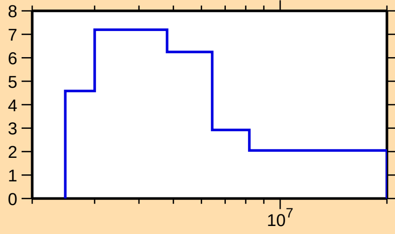
\Delta\sigma/\sigma vs. E for ^{181}\text{Lu}(n,\text{tot.})
