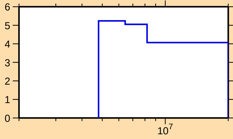
\Delta\sigma/\sigma vs. E for ^{181}\text{Lu}(n,\text{nonel.})
