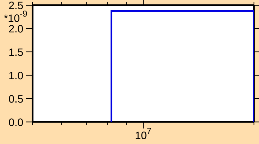
\sigma vs. E for ^{181}\text{Lu}(n,2np)
