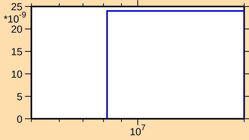
\sigma vs. E for ^{181}\text{Lu}(n,\text{nd})
