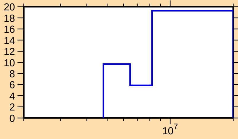
\Delta\sigma/\sigma vs. E for ^{181}\text{Lu}(n,2n)
