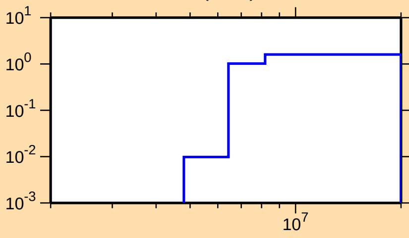
\sigma vs. E for ^{181}\text{Lu}(n,2n)
