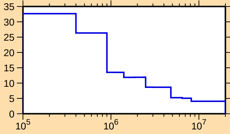
\Delta\sigma/\sigma vs. E for ^{181}\text{Lu}(n,\text{nonel.})
