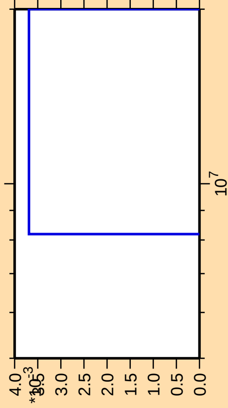
\Delta\sigma/\sigma vs. E for ^{182}\text{Lu}(\text{mt } 11)
