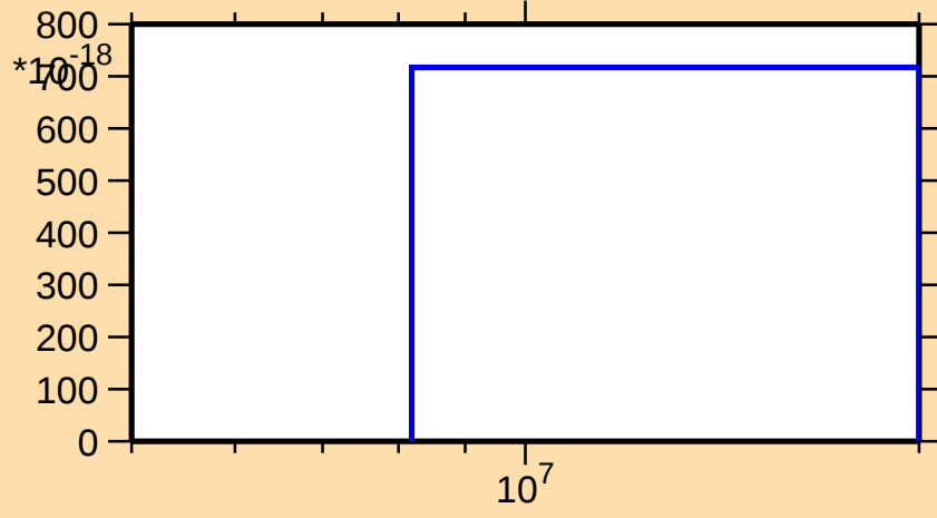
\sigma vs. E for ^{182}\text{Lu}(\text{mt } 11)
