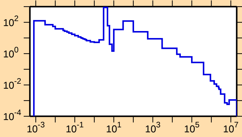
\sigma vs. E for ^{182}\text{Lu}(n,\gamma)
