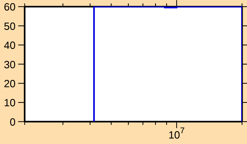
\Delta\sigma/\sigma vs. E for ^{183}\text{Lu}(n,\gamma)
