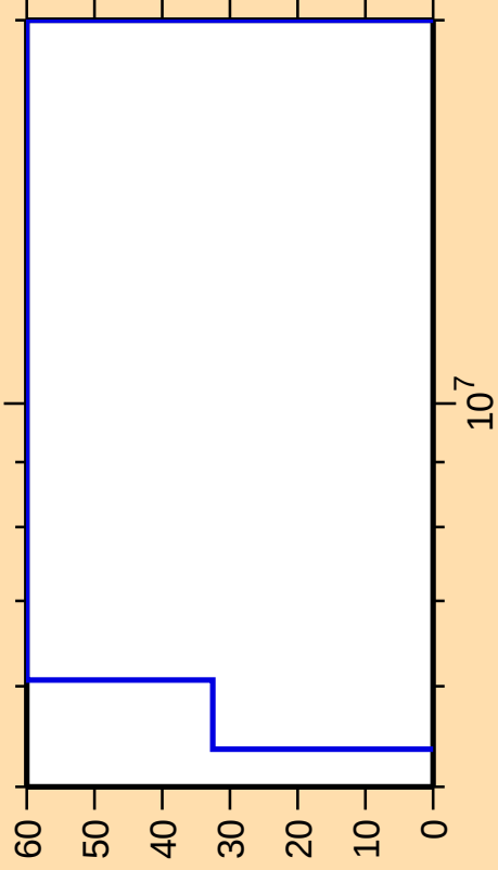
\Delta\sigma/\sigma vs. E for ^{183}\text{Lu}(n,n\text{cont.})
