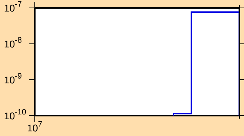
\sigma vs. E for ^{183}\text{Lu}(n,2np)
