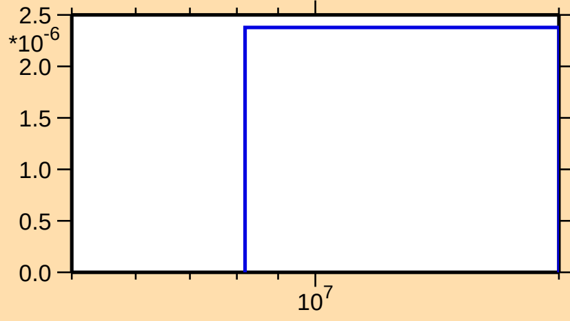
\sigma vs. E for ^{183}\text{Lu}(n,n\alpha)
