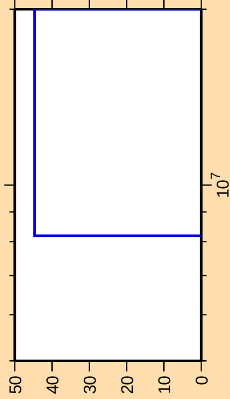
\Delta\sigma/\sigma vs. E for ^{183}\text{Lu}(n,n\alpha)
