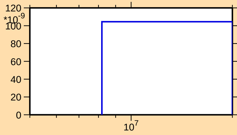
\sigma vs. E for ^{183}\text{Lu}(n,nt)
