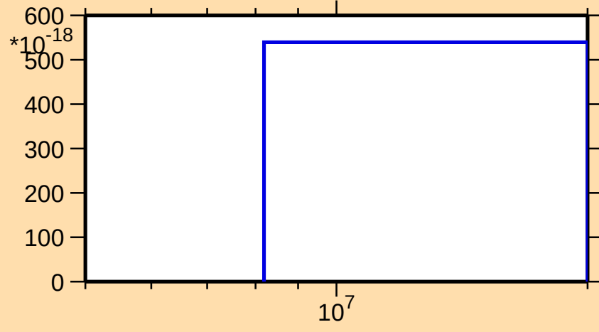
\sigma vs. E for ^{183}\text{Lu}(\text{mt } 11)
