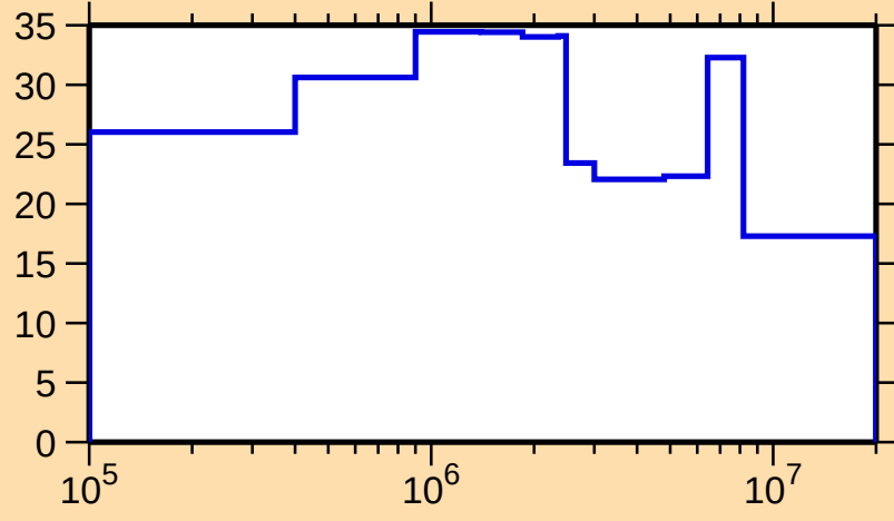
\Delta\sigma/\sigma vs. E for ^{183}\text{Lu}(n,\text{el.})
