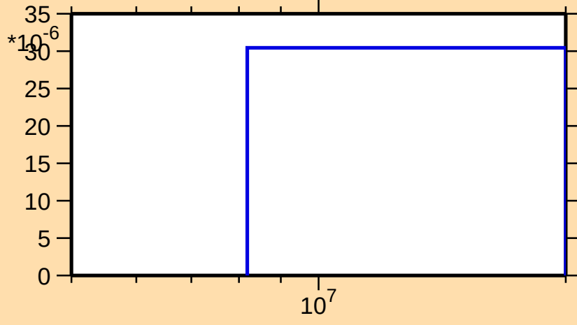
\sigma vs. E for ^{183}\text{Lu}(n,np)
