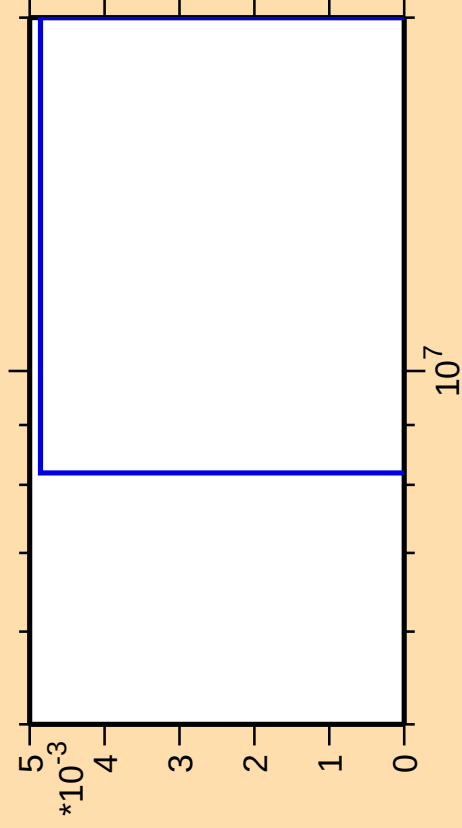
\Delta\sigma/\sigma vs. E for ^{183}\text{Lu}(\text{mt } 11)
