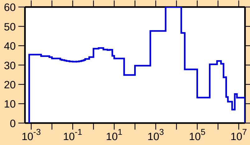
\Delta\sigma/\sigma vs. E for ^{183}\text{Lu}(n,\text{tot.})
