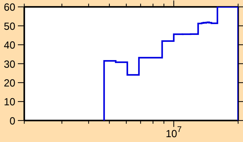
\Delta\sigma/\sigma vs. E for ^{184}\text{Lu}(n,2n)
