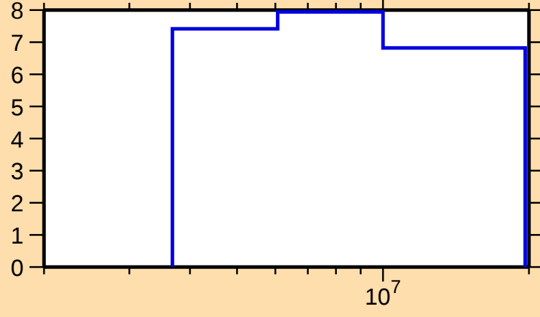
\Delta\sigma/\sigma vs. E for ^{184}\text{Lu}(n,\text{nonel.})
