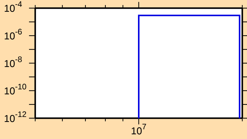
\sigma vs. E for ^{184}\text{Lu}(n,np)
