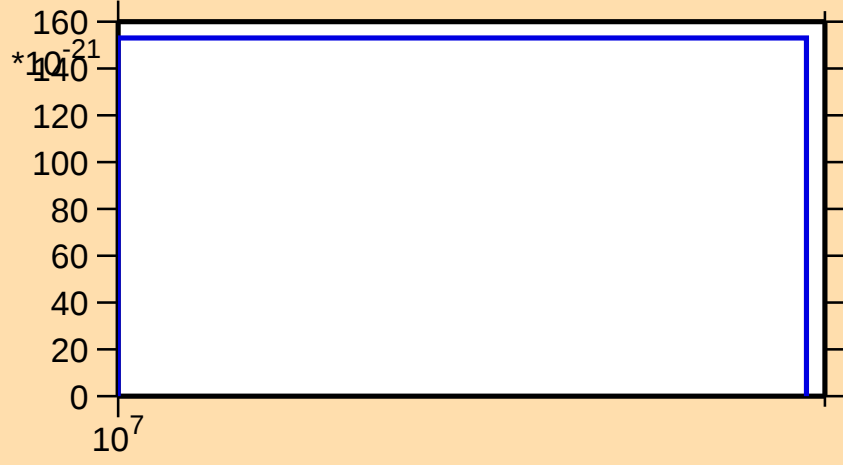
\sigma vs. E for ^{184}\text{Lu} (mt 42)
