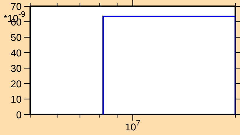
\sigma vs. E for ^{184}\text{Lu}(n,\text{nd})
