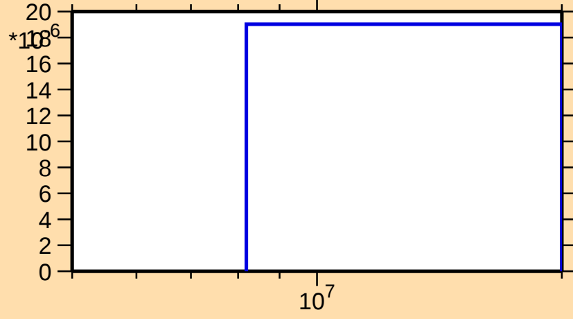
\sigma vs. E for ^{184}\text{Lu}(n,t)
