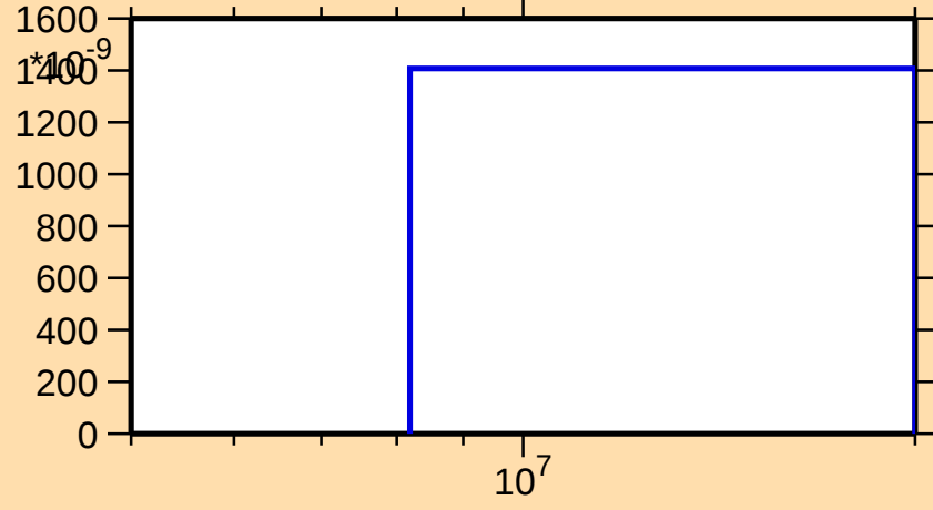
\sigma vs. E for ^{184}\text{Lu}(n,n\alpha)
