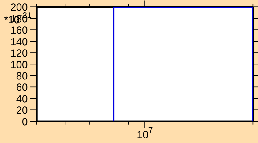
\sigma vs. E for ^{184}\text{Lu}(\text{mt } 42)
