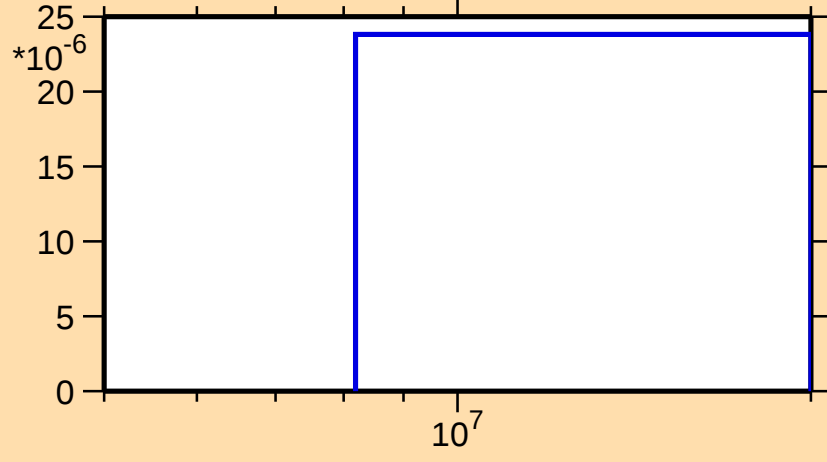
\sigma vs. E for ^{184}\text{Lu}(n,np)
