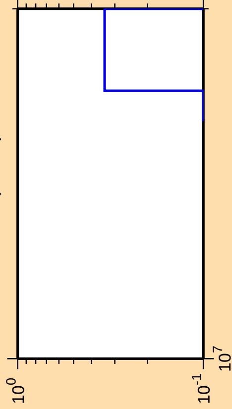
\Delta\sigma/\sigma vs. E for ^{185}\text{Lu} (mt 11)
