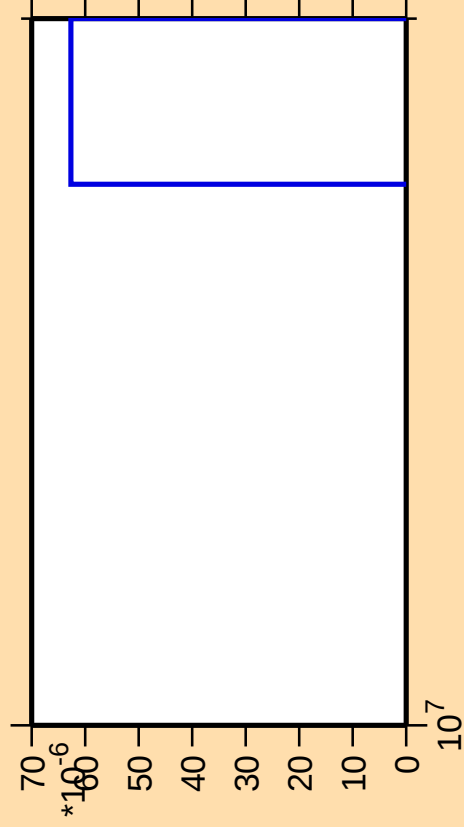
\Delta\sigma/\sigma vs. E for ^{185}\text{Lu} (mt 42)
