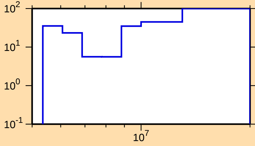
\Delta\sigma/\sigma vs. E for ^{185}\text{Lu}(n,2n)
