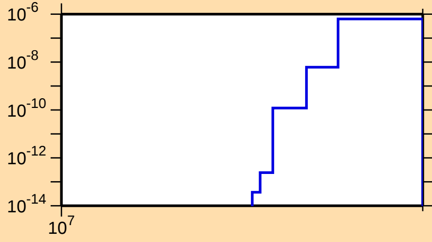
\sigma vs. E for ^{185}\text{Lu}(n,\text{nd})
