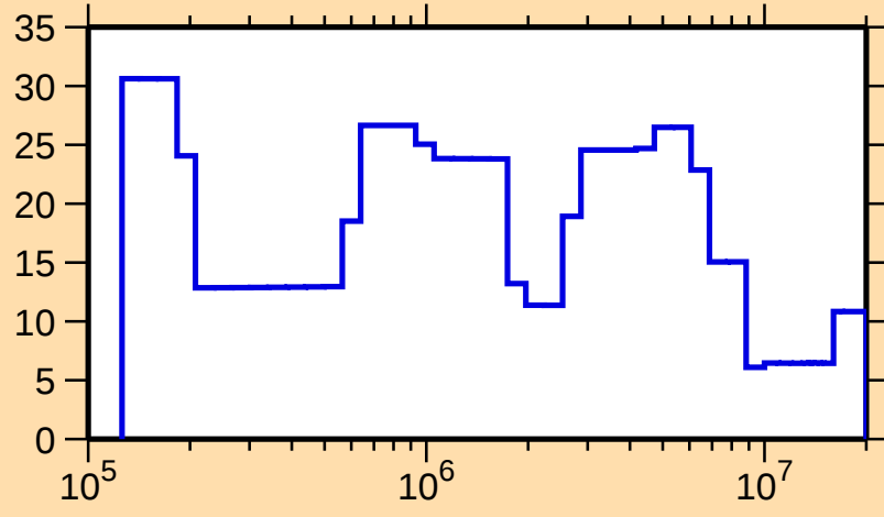
\Delta\sigma/\sigma vs. E for ^{185}\text{Lu}(n,\text{el.})
