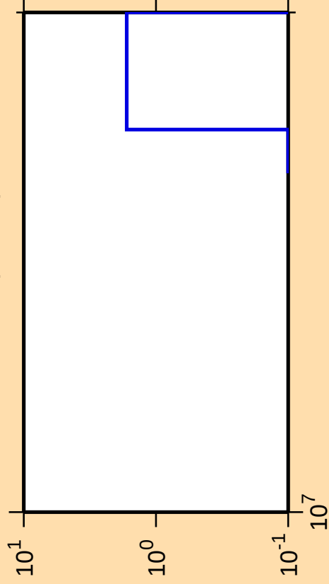
\Delta\sigma/\sigma vs. E for ^{185}\text{Lu}(n,3n\alpha)
