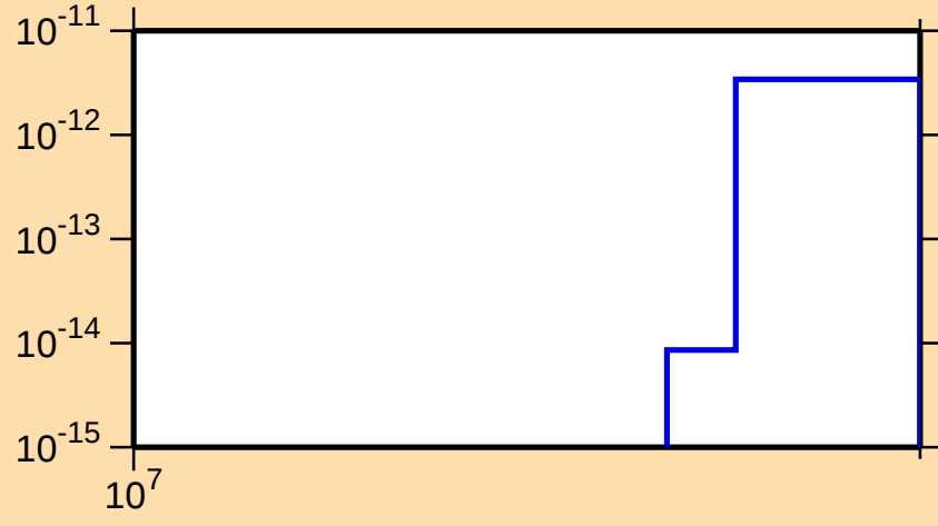
\sigma vs. E for ^{185}\text{Lu}(n,3n\alpha)
