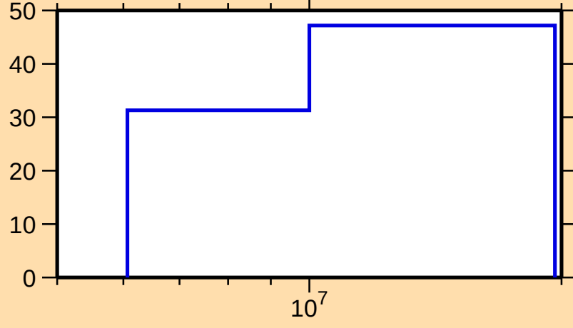
\Delta\sigma/\sigma vs. E for ^{185}\text{Lu}(n,\text{ncont.})
