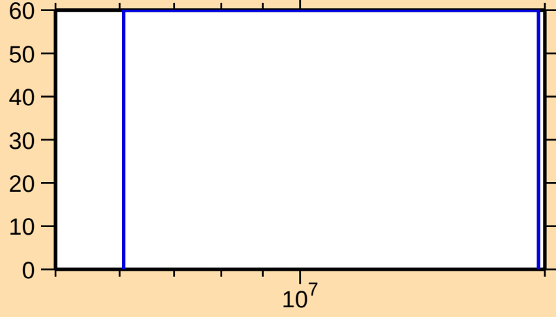
\Delta\sigma/\sigma vs. E for ^{185}\text{Lu}(n,\gamma)
