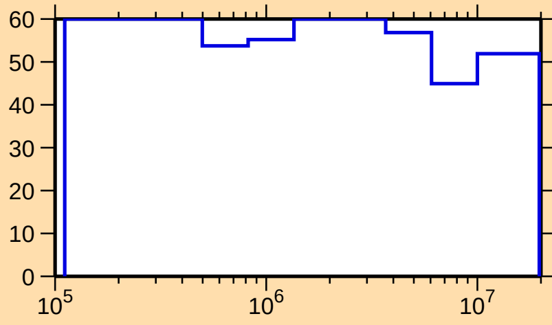
\Delta\sigma/\sigma vs. E for ^{185}\text{Lu}(n,n_1)
