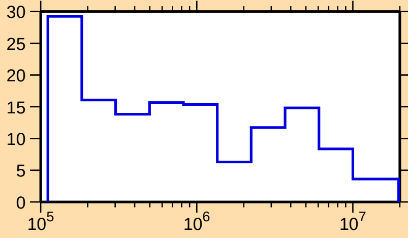
\Delta\sigma/\sigma vs. E for ^{185}\text{Lu}(n,\text{tot.})
