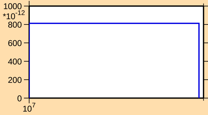
\sigma vs. E for ^{185}\text{Lu}(n,2n\alpha)
