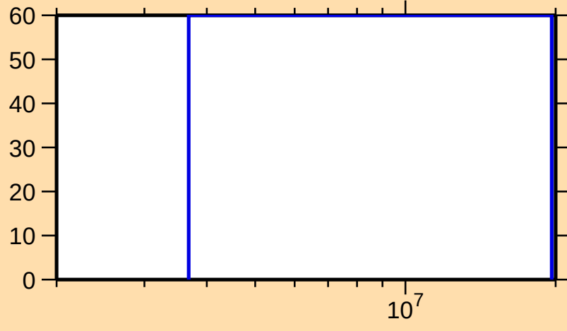
\Delta\sigma/\sigma vs. E for ^{185}\text{Lu}(n,\gamma)
