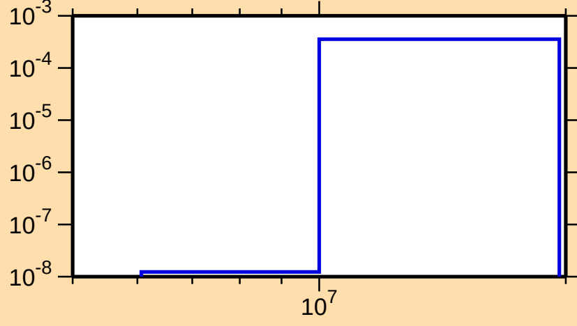
\sigma vs. E for ^{185}\text{Lu}(n,p)
