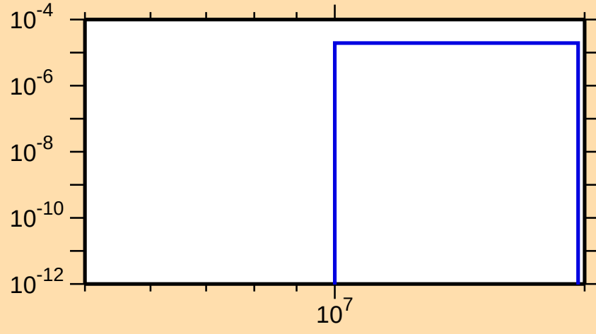
\sigma vs. E for ^{185}\text{Lu}(n,np)
