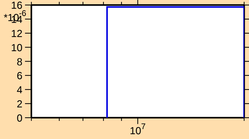
\sigma vs. E for ^{185}\text{Lu}(n,np)
