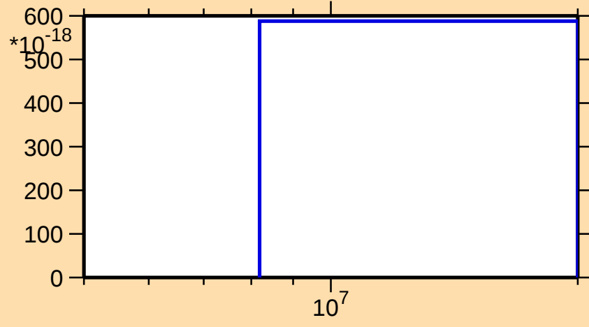
\sigma vs. E for ^{185}\text{Lu} (mt 11)
