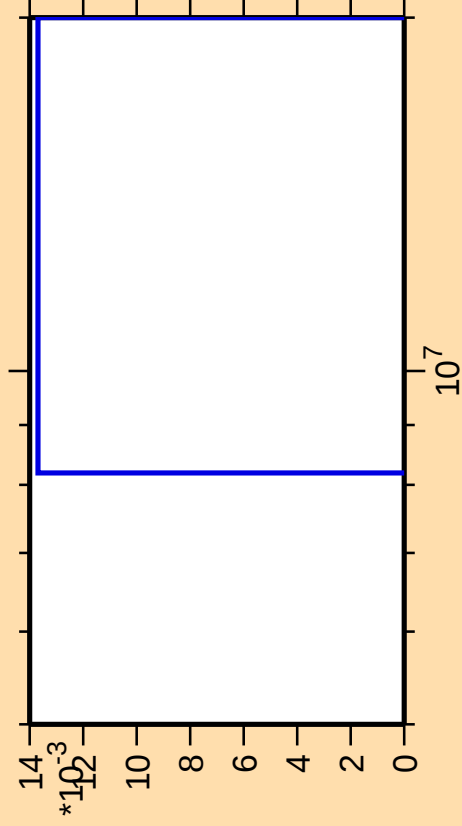
\Delta\sigma/\sigma vs. E for ^{185}\text{Lu}(n,3n\alpha)
