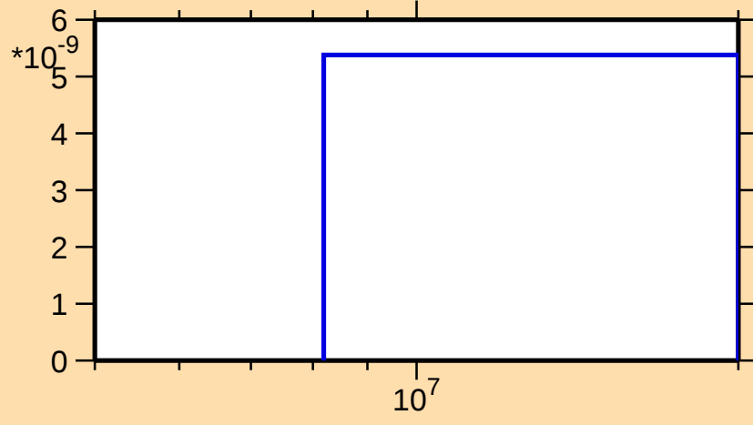
\sigma vs. E for ^{185}\text{Lu}(n,\text{nd})
