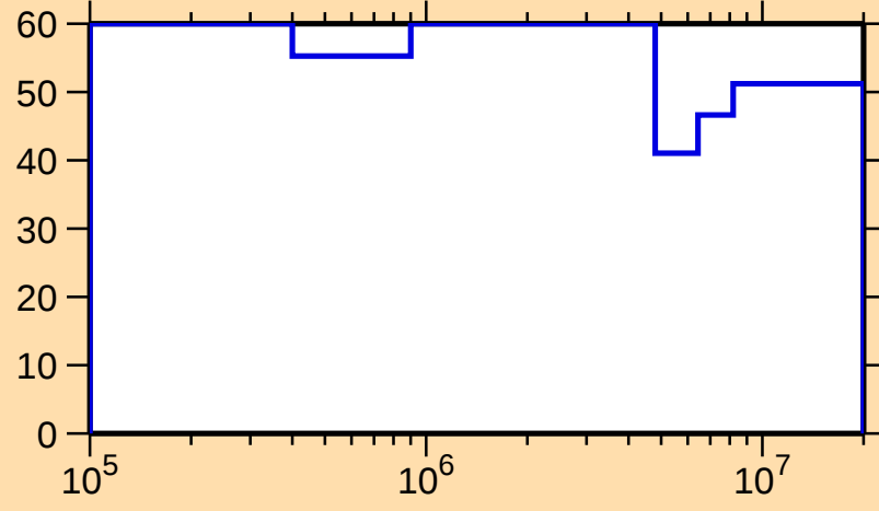
\Delta\sigma/\sigma vs. E for ^{185}\text{Lu}(n,n_1)
