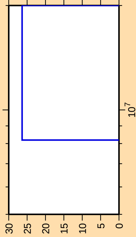
\Delta\sigma/\sigma vs. E for ^{185}\text{Lu}(n,3n)
