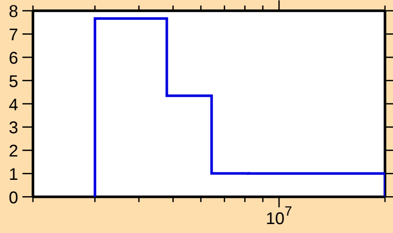
\Delta\sigma/\sigma vs. E for ^{185}\text{Lu}(n,\text{nonel.})
