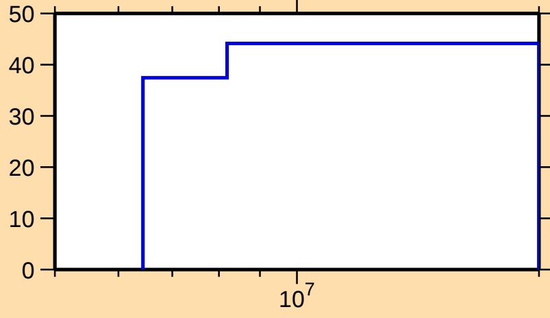
\Delta\sigma/\sigma vs. E for ^{185}\text{Lu}(n,n\text{cont.})
