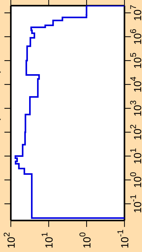
\Delta\sigma/\sigma vs. E for ^{185}\text{Lu}(n,\text{nonel.})
