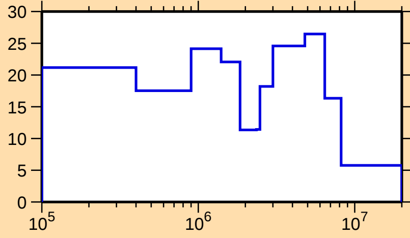
\Delta\sigma/\sigma vs. E for ^{185}\text{Lu}(n,\text{el.})
