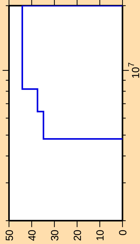
\Delta\sigma/\sigma vs. E for ^{185}\text{Lu}(n,n\text{cont.})
