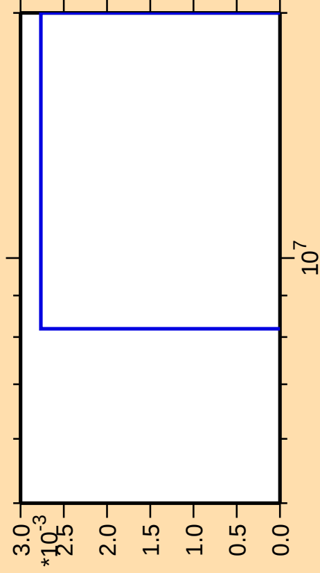
\Delta\sigma/\sigma vs. E for ^{185}\text{Lu} (mt 11)
