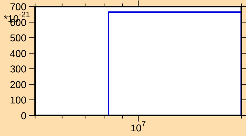
\sigma vs. E for ^{185}\text{Lu} (mt 42)
