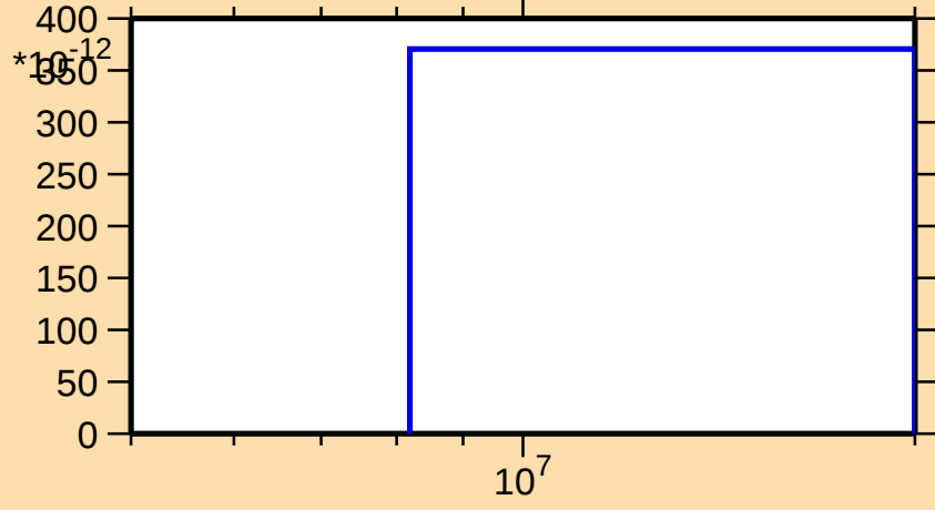
\sigma vs. E for ^{185}\text{Lu}(n,2np)
