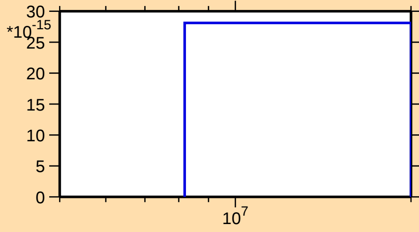
\sigma vs. E for ^{185}\text{Lu}(n,3n\alpha)
