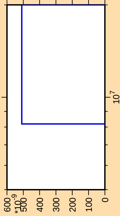
\Delta\sigma/\sigma vs. E for ^{185}\text{Lu} (mt 42)
