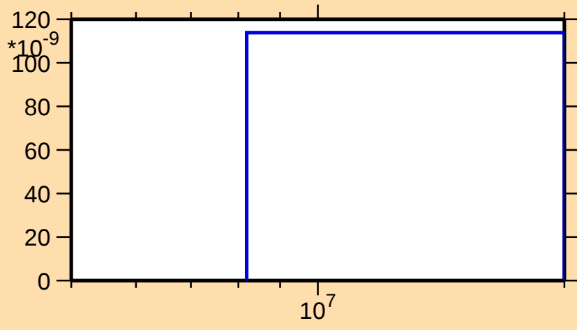
\sigma vs. E for ^{185}\text{Lu}(n,nt)
