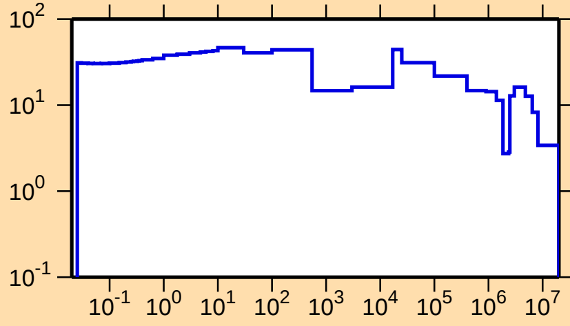
\Delta\sigma/\sigma vs. E for ^{185}\text{Lu}(n,\text{tot.})
