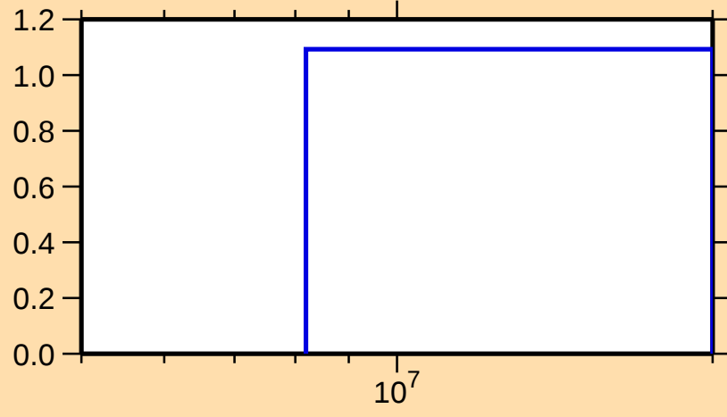
\sigma vs. E for ^{185}\text{Lu}(n,3n)
