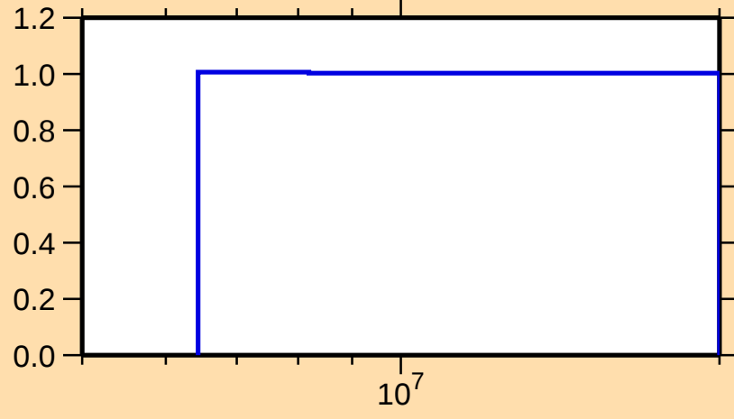
\Delta\sigma/\sigma vs. E for ^{185}\text{Lu}(n,\text{nonel.})
