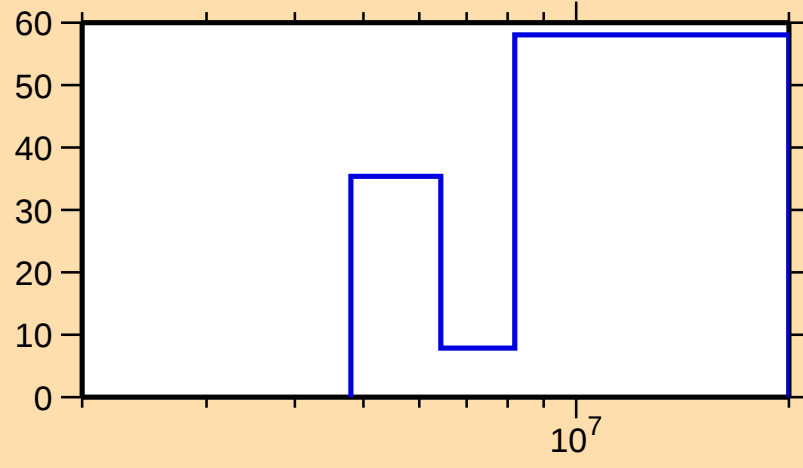
\Delta\sigma/\sigma vs. E for ^{185}\text{Lu}(n,2n)
