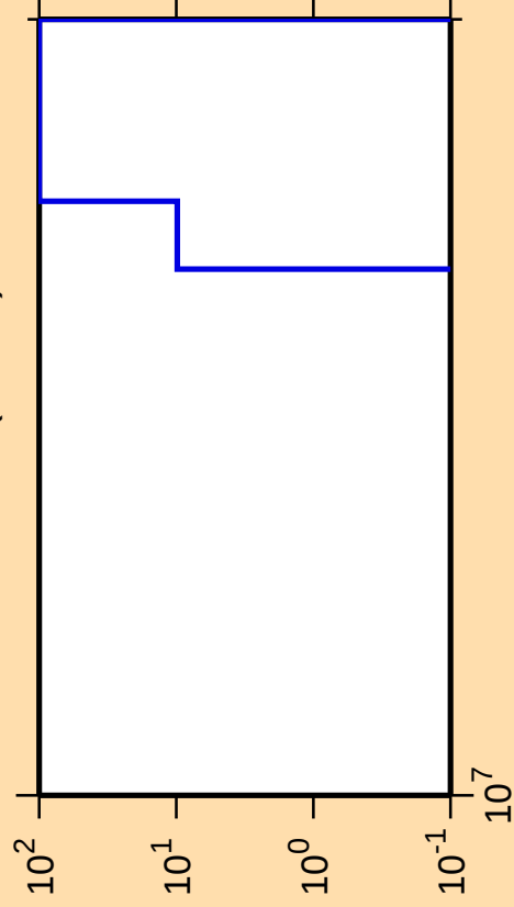
\Delta\sigma/\sigma vs. E for ^{247}\text{Md}(\text{mt } 34)
