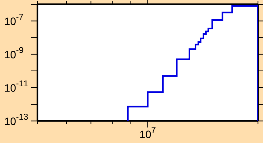
\sigma vs. E for ^{247}\text{Md}(\text{mt117})
