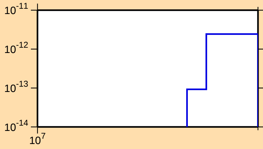
\sigma vs. E for ^{247}\text{Md}(n,\text{pt})
