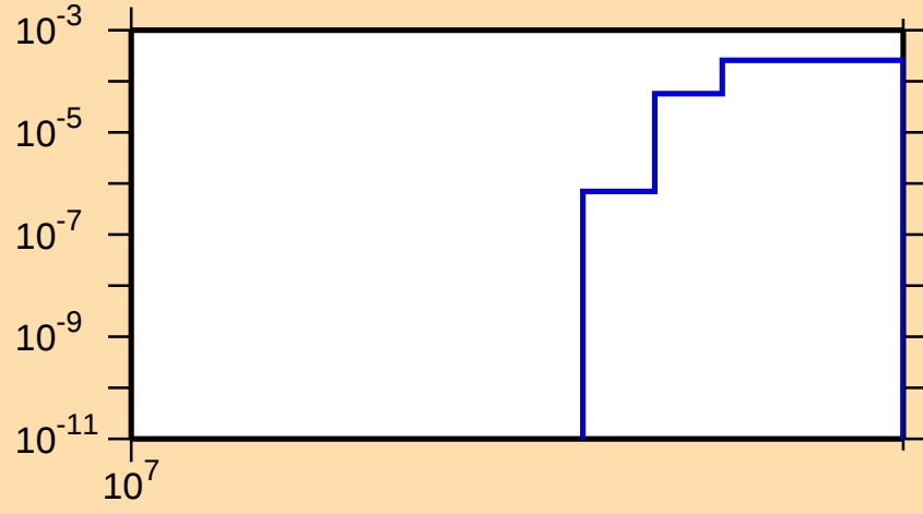
\sigma vs. E for ^{247}\text{Md}(n,3n\alpha)
