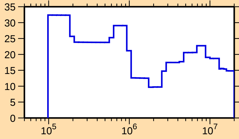
\Delta\sigma/\sigma vs. E for ^{247}\text{Md}(n,\text{tot.})
