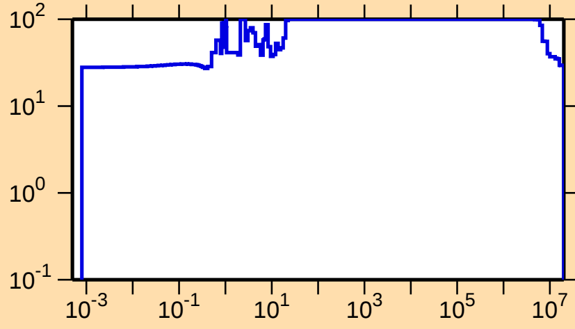
\Delta\sigma/\sigma vs. E for ^{247}\text{Md}(n,f)
