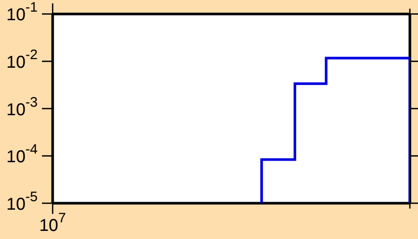
\sigma vs. E for ^{247}\text{Md}(n,3n)
