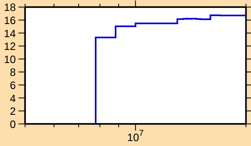
\Delta\sigma/\sigma vs. E for ^{247}\text{Md}(n,\text{nonel.})
