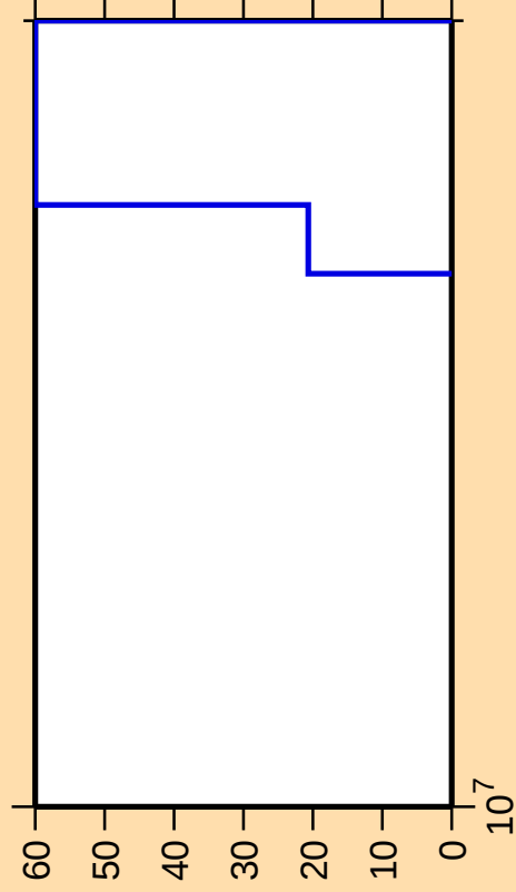
\Delta\sigma/\sigma vs. E for ^{247}\text{Md}(n,\text{pd})
