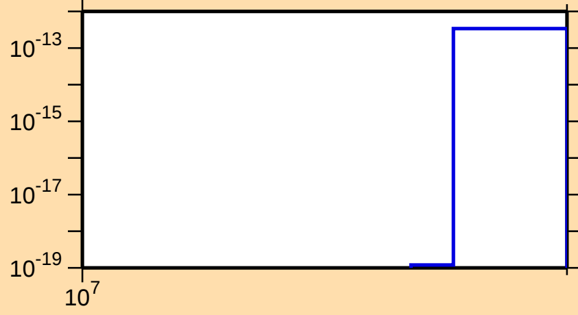
\sigma vs. E for ^{247}\text{Md}(\text{mt } 11)
