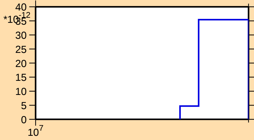
\sigma vs. E for ^{247}\text{Md}(n,\text{pd})
