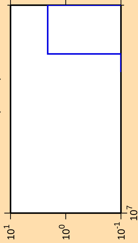
\Delta\sigma/\sigma vs. E for ^{247}\text{Md}(\text{mt } 11)
