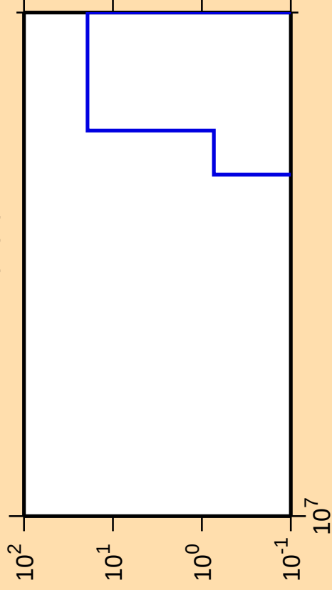
\Delta\sigma/\sigma vs. E for ^{247}\text{Md}(n,\text{pt})
