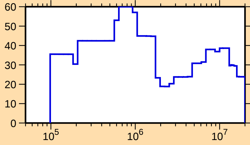
\Delta\sigma/\sigma vs. E for ^{247}\text{Md}(n,\text{el.})
