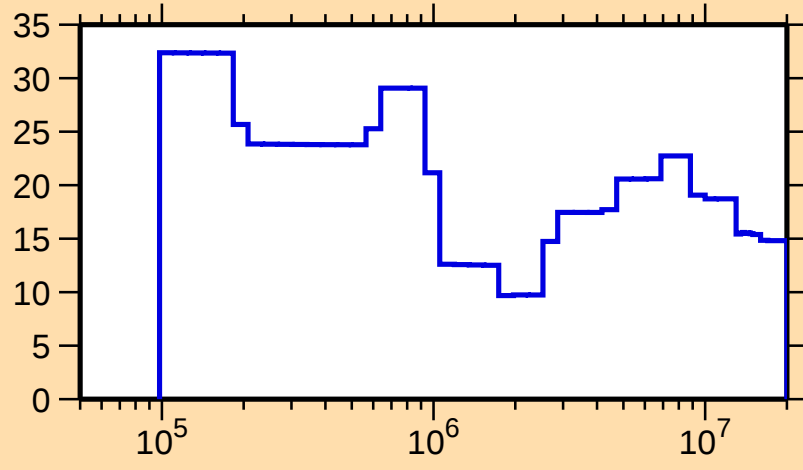
\Delta\sigma/\sigma vs. E for ^{247}\text{Md}(n,\text{tot.})
