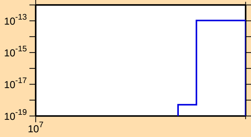
\sigma vs. E for ^{247}\text{Md}(\text{mt } 42)
