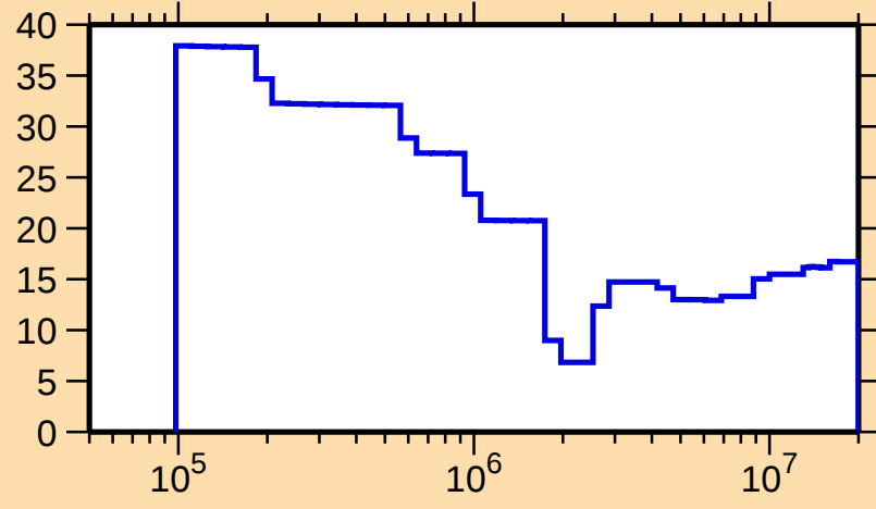
\Delta\sigma/\sigma vs. E for ^{247}\text{Md}(n,\text{nonel.})
