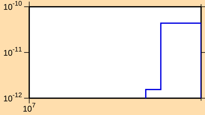
\sigma vs. E for ^{247}\text{Md}(\text{mt } 34)
