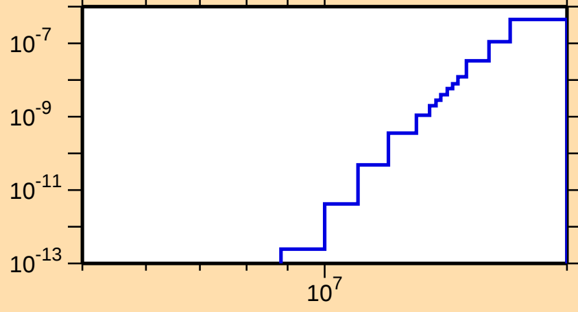
\sigma vs. E for ^{247}\text{Md}(n,\text{He3})
