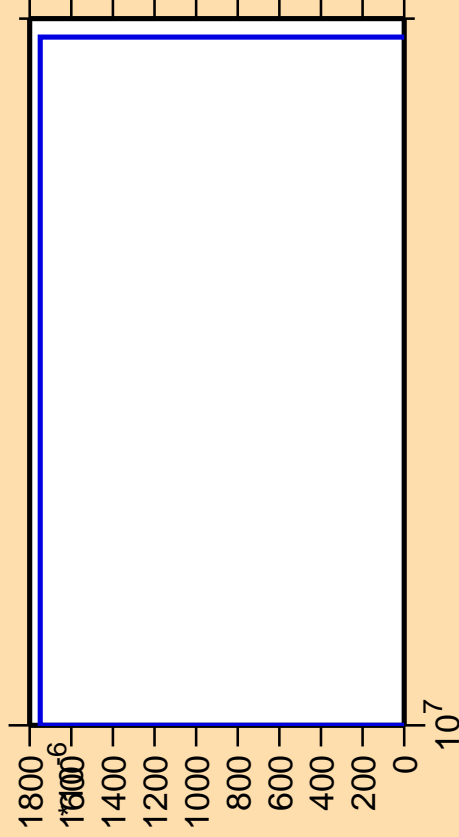
\Delta\sigma/\sigma vs. E for ^{247}\text{Md} (mt 42)
