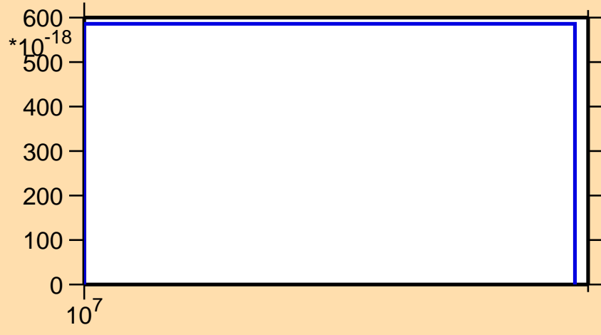
\sigma vs. E for ^{247}\text{Md} (mt 42)
