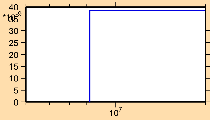
\sigma vs. E for ^{247}\text{Md}(\text{mt117})
