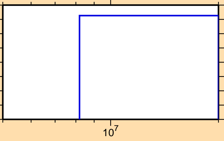
\sigma vs. E for ^{247}\text{Md}(n,nt)
