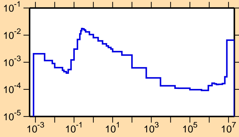
\sigma vs. E for ^{247}\text{Md}(n,\alpha)
