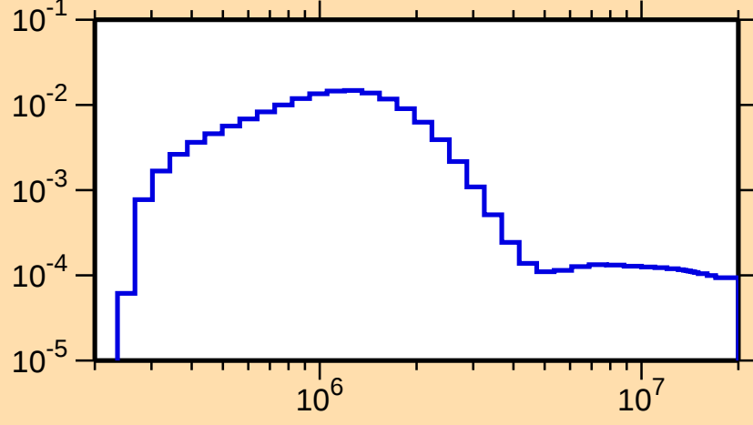
\sigma vs. E for ^{249}\text{Md}(n,n_4)
