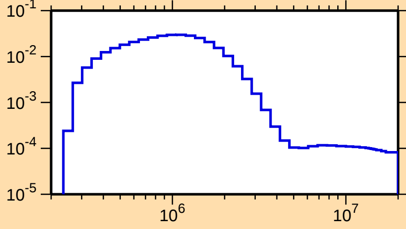
\sigma vs. E for ^{249}\text{Md}(n,n_3)
