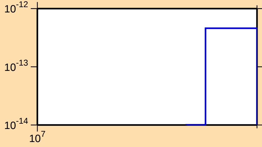
\sigma vs. E for ^{249}\text{Md}(n,\text{pt})
