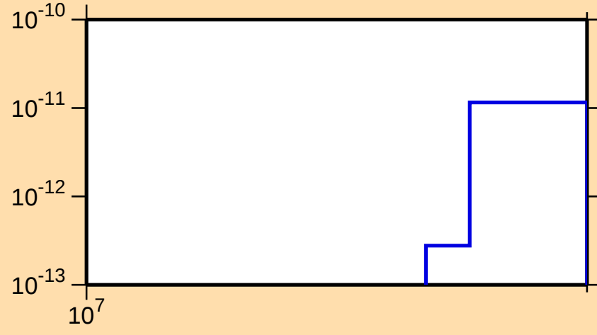
\sigma vs. E for ^{249}\text{Md}(\text{mt } 34)
