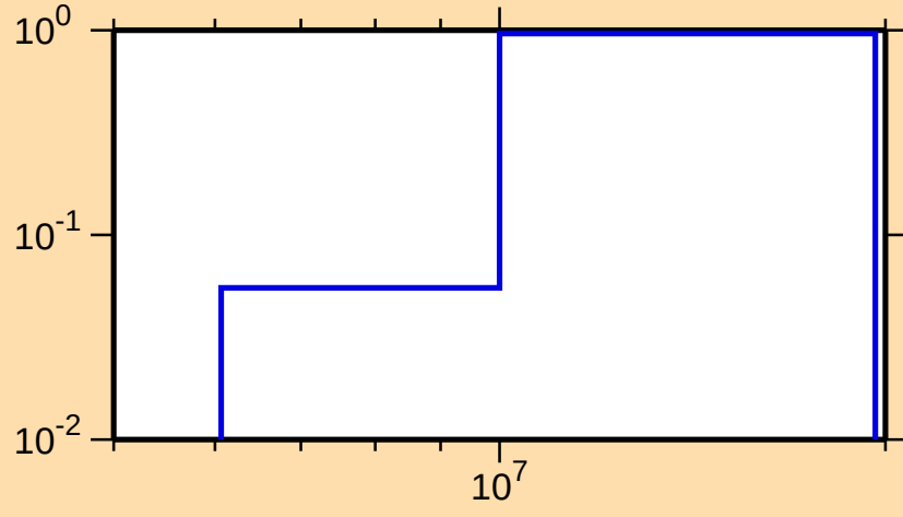
\sigma vs. E for ^{249}\text{Md}(n,2n)
