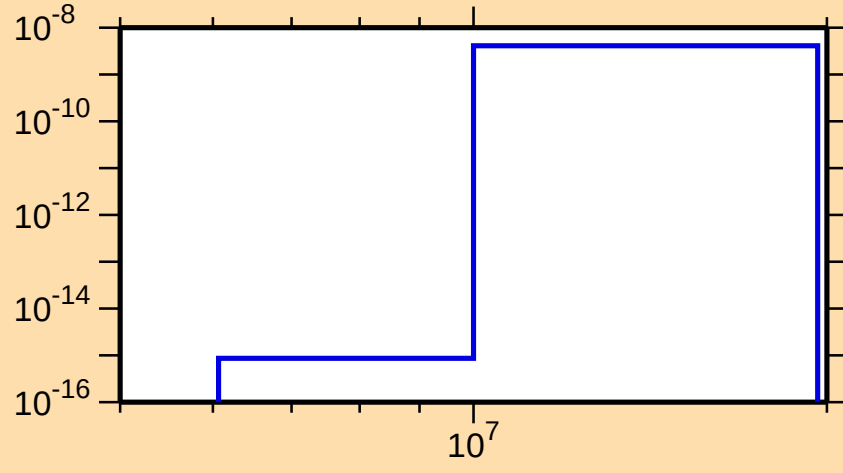
\sigma vs. E for ^{249}\text{Md}(n,\text{He3})
