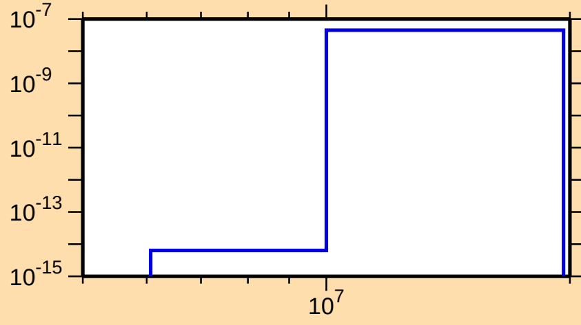
\sigma vs. E for ^{249}\text{Md}(\text{mt } 45)
