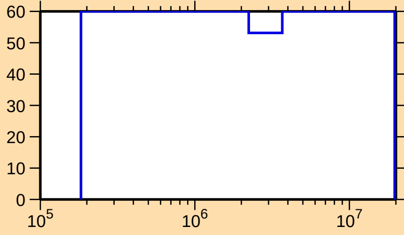
\Delta\sigma/\sigma vs. E for ^{249}\text{Md}(n,n_1)
