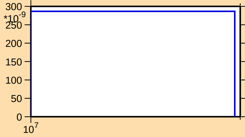
\sigma vs. E for ^{249}\text{Md}(n,2np)
