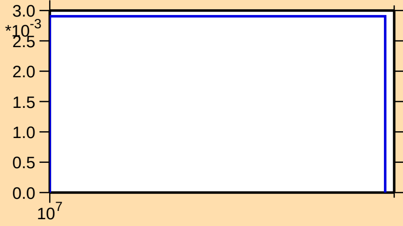
\sigma vs. E for ^{249}\text{Md}(n,3n)
