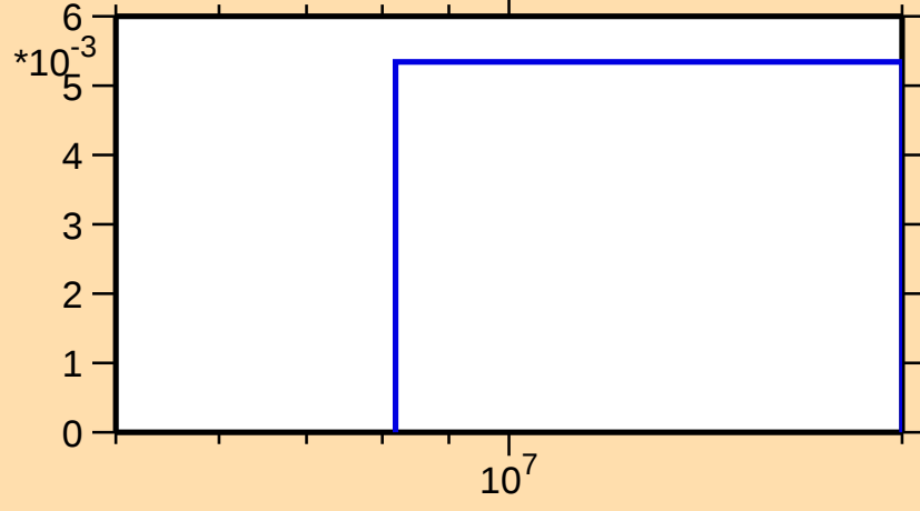
\sigma vs. E for ^{249}\text{Md}(n,3n\alpha)
