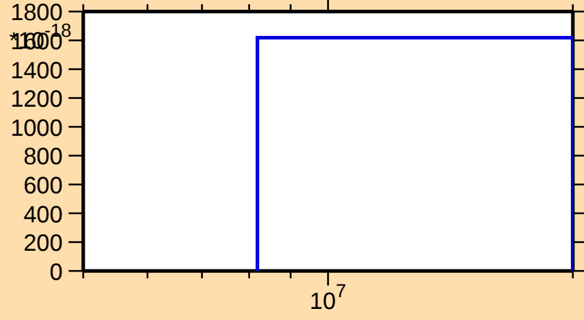
\sigma vs. E for ^{249}\text{Md}(\text{mt } 42)
