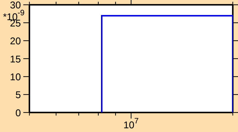
\sigma vs. E for ^{249}\text{Md}(n,\text{nt})
