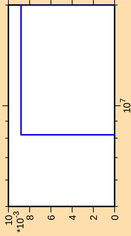
\Delta\sigma/\sigma vs. E for ^{249}\text{Md}(\text{mt } 42)
