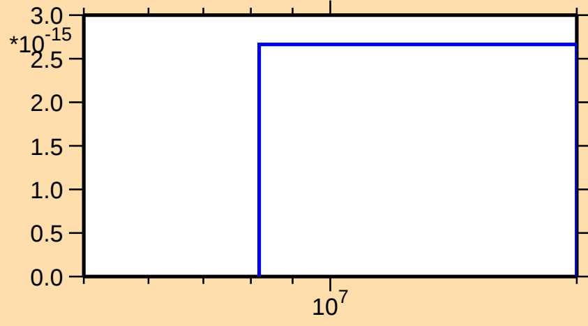
\sigma vs. E for ^{249}\text{Md}(\text{mt } 11)
