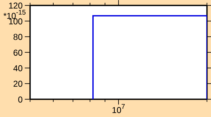
\sigma vs. E for ^{249}\text{Md}(\text{mt } 34)
