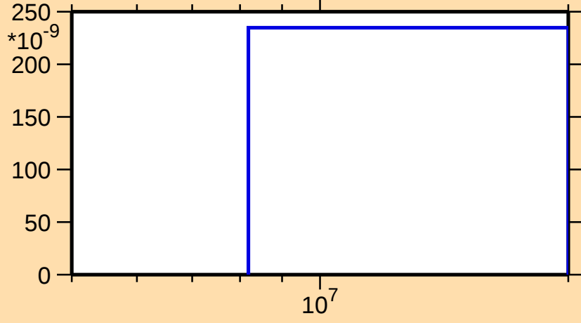
\sigma vs. E for ^{249}\text{Md}(n,2np)
