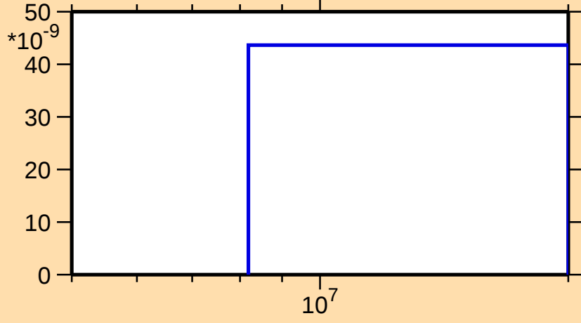
\sigma vs. E for ^{249}\text{Md}(\text{mt117})
