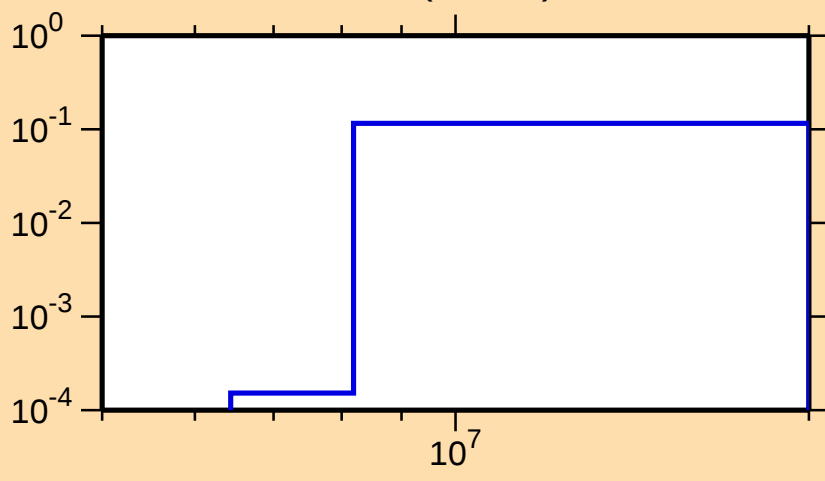
\sigma vs. E for ^{249}\text{Md}(n,2n\alpha)
