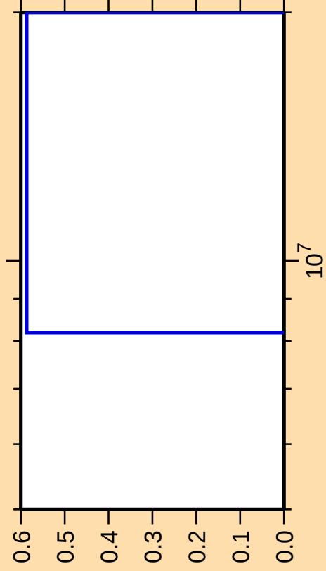
\Delta\sigma/\sigma vs. E for ^{249}\text{Md}(\text{mt } 34)
