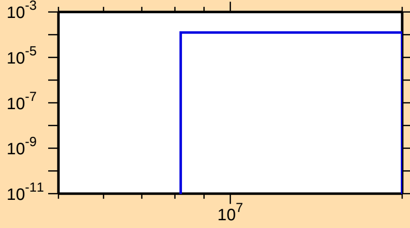
\sigma vs. E for ^{249}\text{Md}(n,t)
