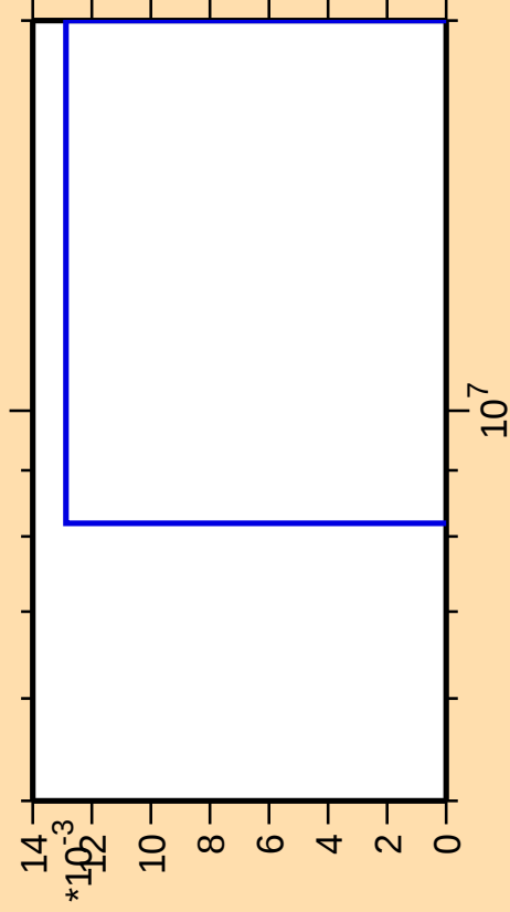
\Delta\sigma/\sigma vs. E for ^{249}\text{Md}(\text{mt } 11)
