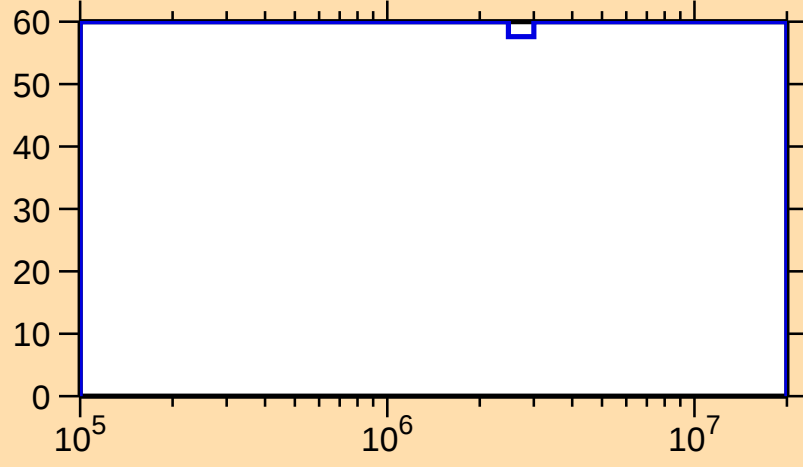
\Delta\sigma/\sigma vs. E for ^{249}\text{Md}(n,n_1)
