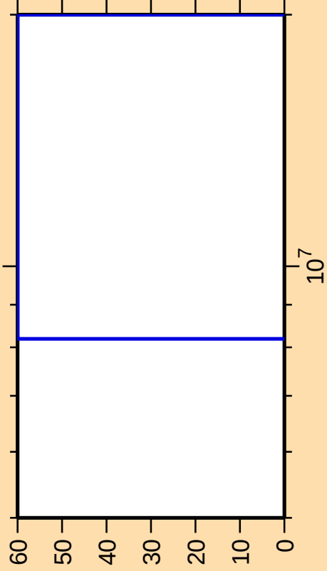
\Delta\sigma/\sigma vs. E for ^{249}\text{Md}(n,\text{nt})
