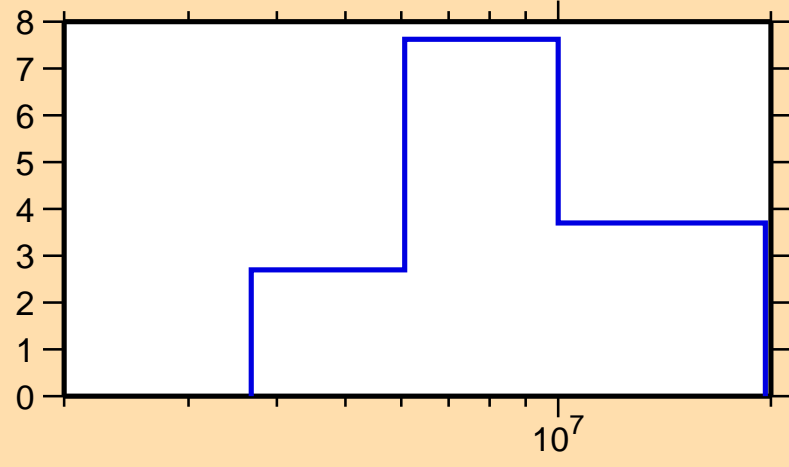
\Delta\sigma/\sigma vs. E for ^{254}\text{Md}(n,\text{tot.})
