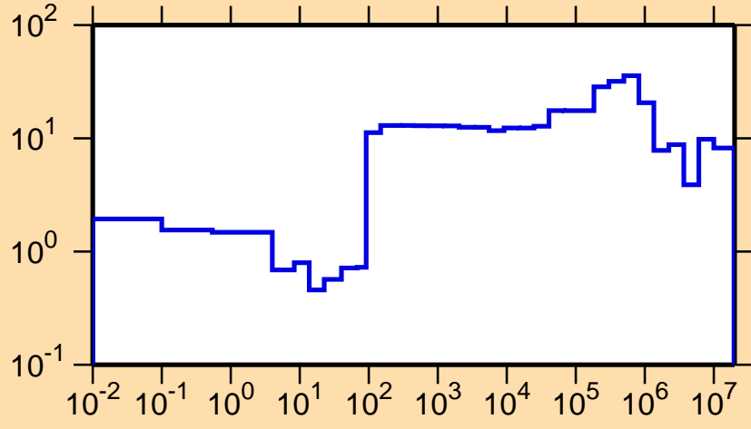
\Delta\sigma/\sigma vs. E for ^{254}\text{Md}(n,el.)
