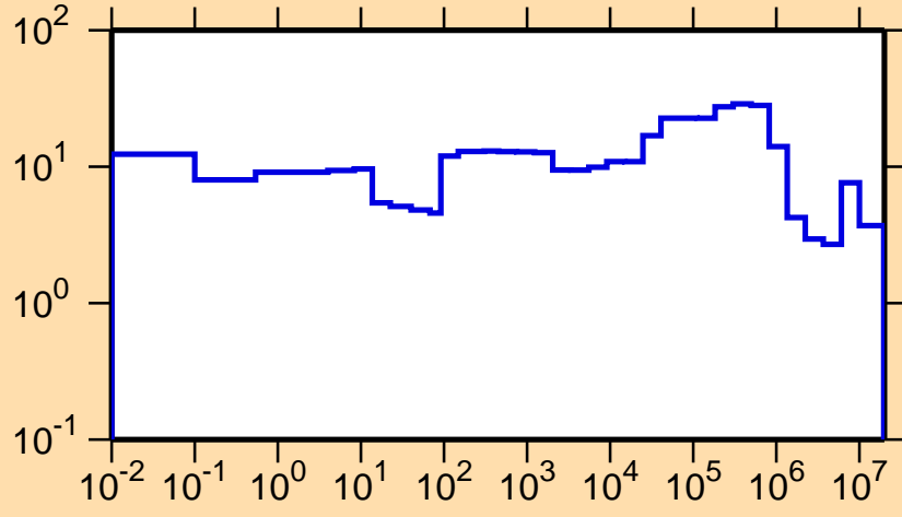
\Delta\sigma/\sigma vs. E for ^{254}\text{Md}(n,tot.)
