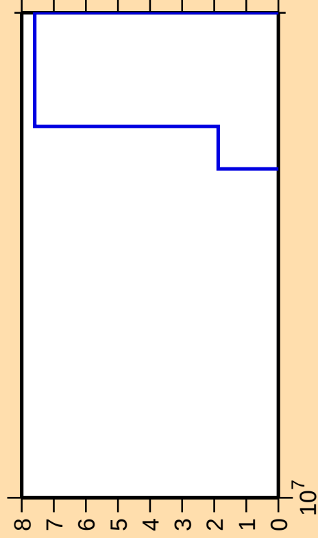
\Delta\sigma/\sigma vs. E for ^{254}\text{Md}(\text{mt117})
