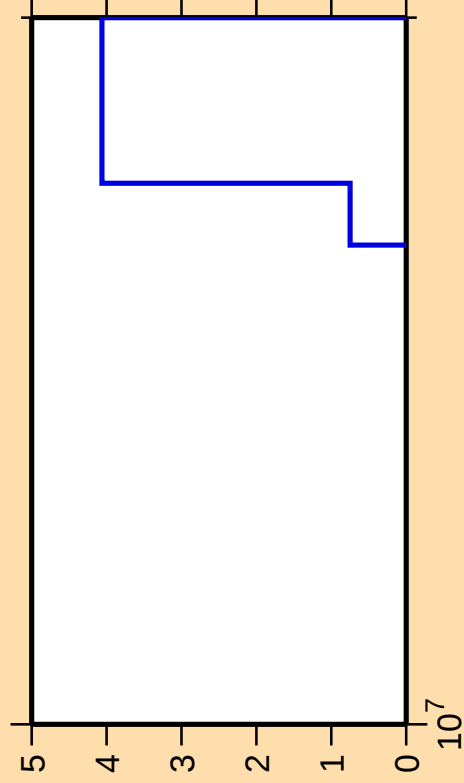
\Delta\sigma/\sigma vs. E for ^{254}\text{Md}(\text{mt } 45)
