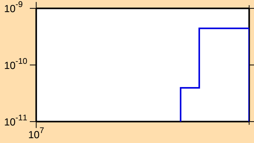
\sigma vs. E for ^{257}\text{Md}(n,\text{He}3)
