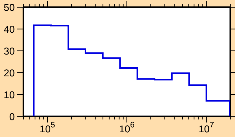
\Delta\sigma/\sigma vs. E for ^{257}\text{Md}(n,\text{tot.})
