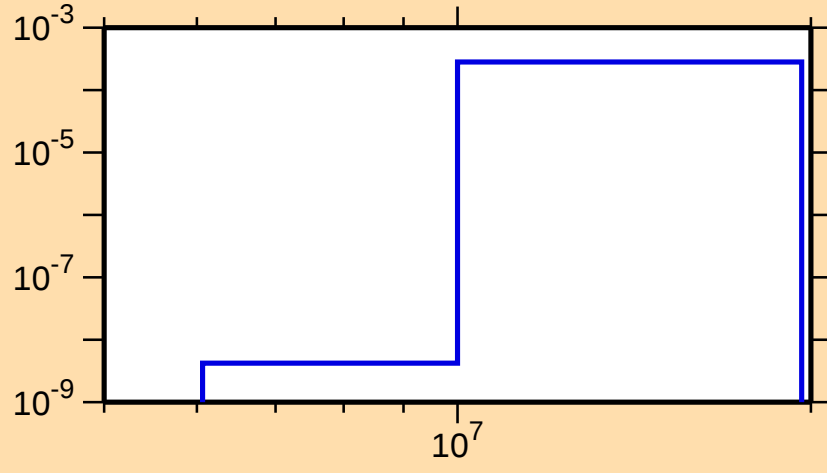
\sigma vs. E for ^{257}\text{Md}(n,d)
