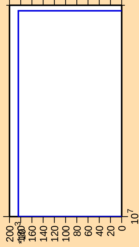
\Delta\sigma/\sigma vs. E for ^{257}\text{Md}(\text{mt } 11)
