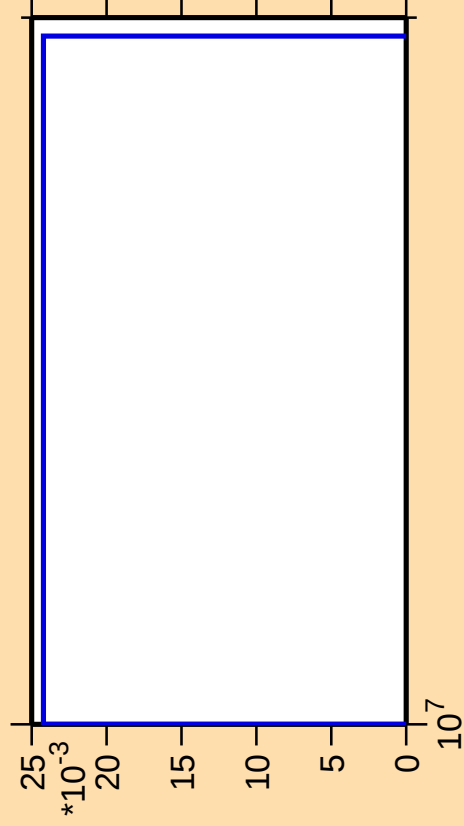
\Delta\sigma/\sigma vs. E for ^{257}\text{Md}(\text{mt } 42)
