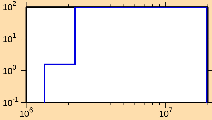
\Delta\sigma/\sigma vs. E for ^{257}\text{Md}(n,p)
