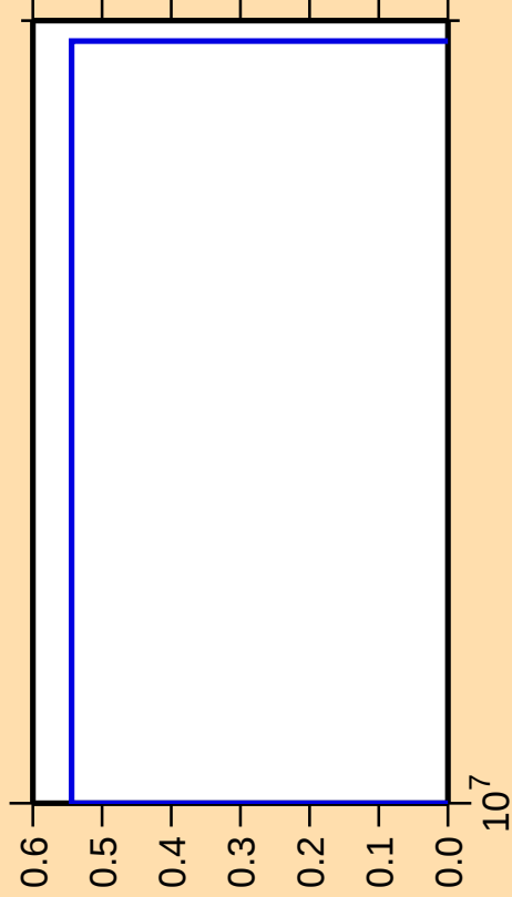
\Delta\sigma/\sigma vs. E for ^{257}\text{Md}(n,p\alpha)
