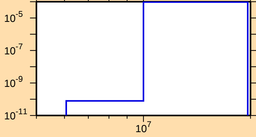
\sigma vs. E for ^{257}\text{Md}(n,t)
