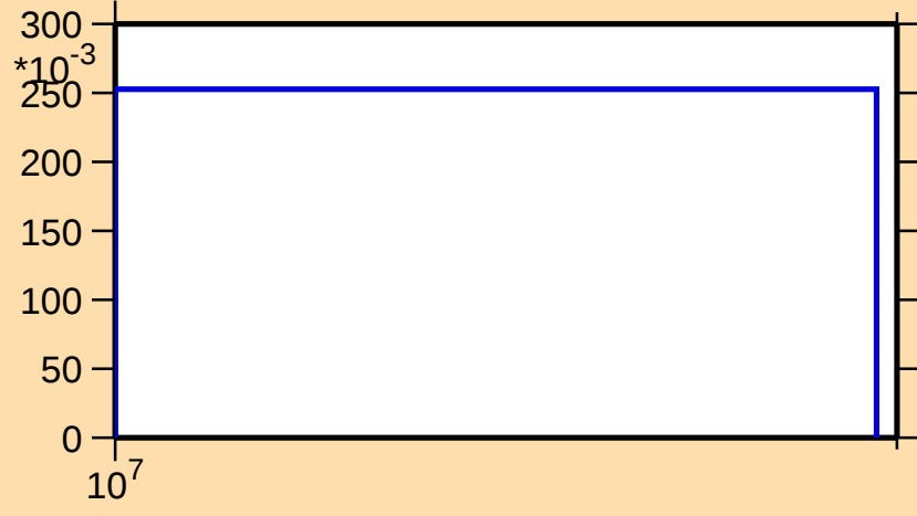
\sigma vs. E for ^{257}\text{Md}(n,3n)
