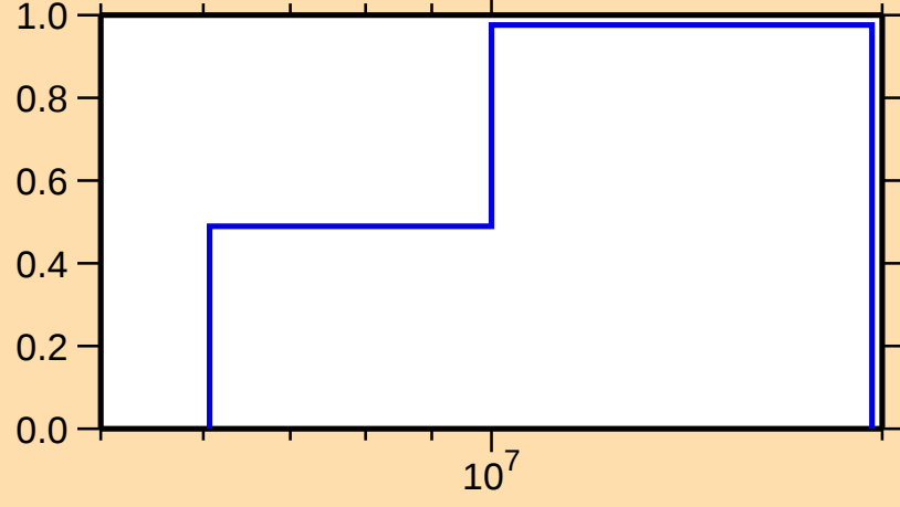
\sigma vs. E for ^{257}\text{Md}(n,2n)
