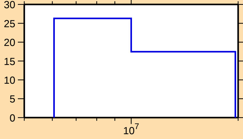
\Delta\sigma/\sigma vs. E for ^{257}\text{Md}(n,\text{el.})
