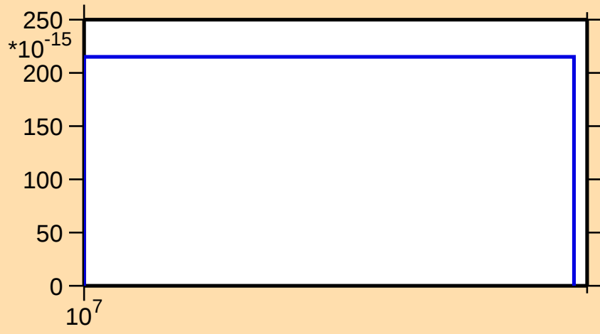
\sigma vs. E for ^{257}\text{Md}(n,p\alpha)
