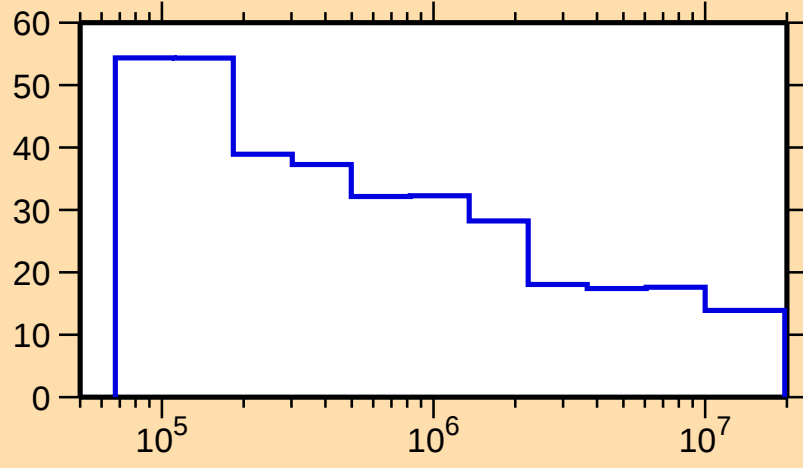
\Delta\sigma/\sigma vs. E for ^{257}\text{Md}(n,\text{nonel.})
