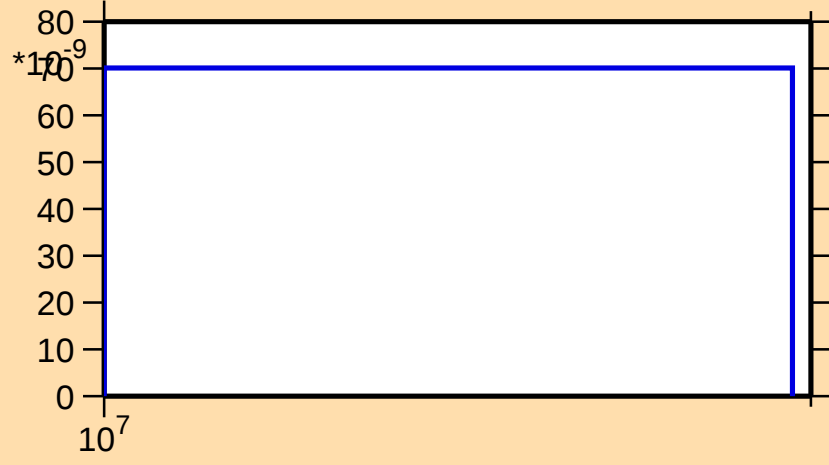
\sigma vs. E for ^{257}\text{Md}(n,3n\alpha)
