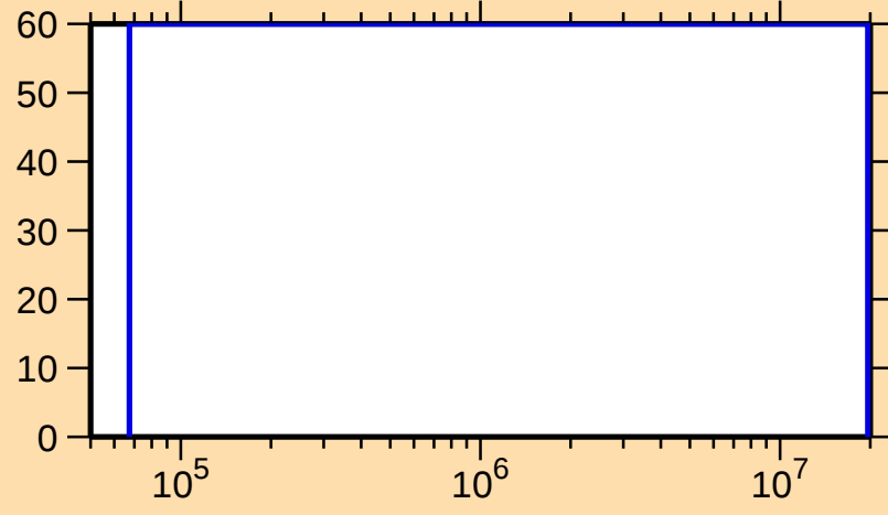
\Delta\sigma/\sigma vs. E for ^{257}\text{Md}(n,f)
