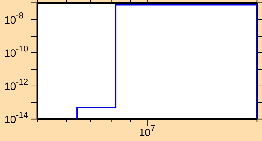
\sigma vs. E for ^{257}\text{Md}(n,2n\alpha)
