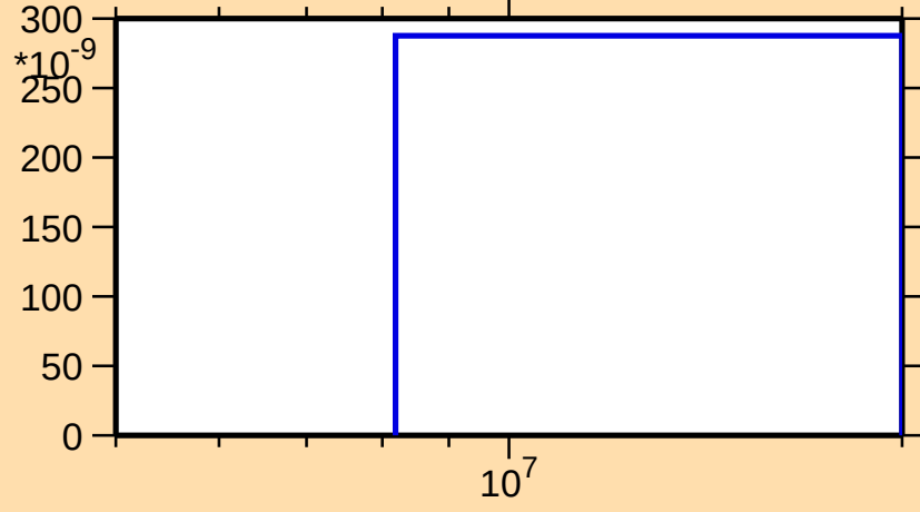
\sigma vs. E for ^{257}\text{Md}(n,\text{nt})
