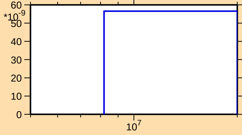
\sigma vs. E for ^{257}\text{Md}(n,3n\alpha)
