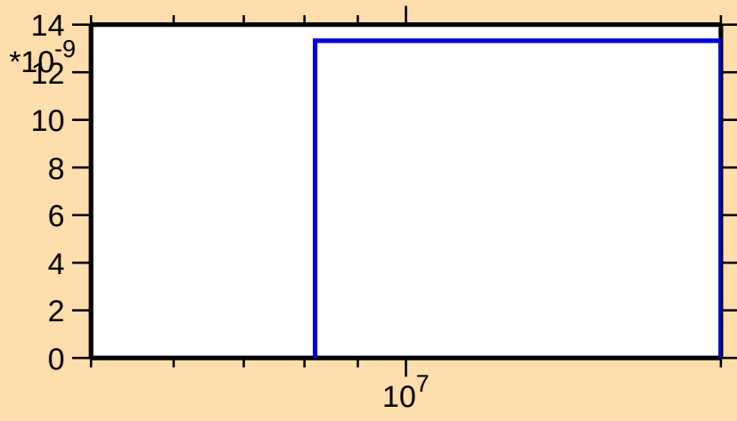
\sigma vs. E for ^{257}\text{Md}(n,2np)
