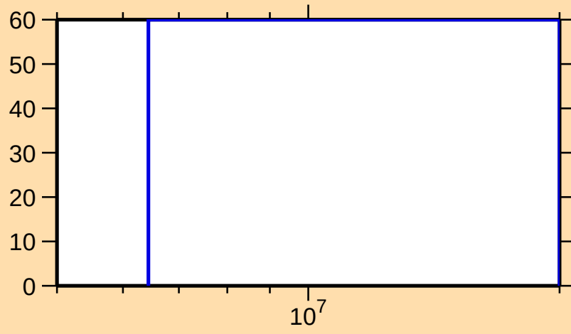
\Delta\sigma/\sigma vs. E for ^{257}\text{Md}(n,2n)
