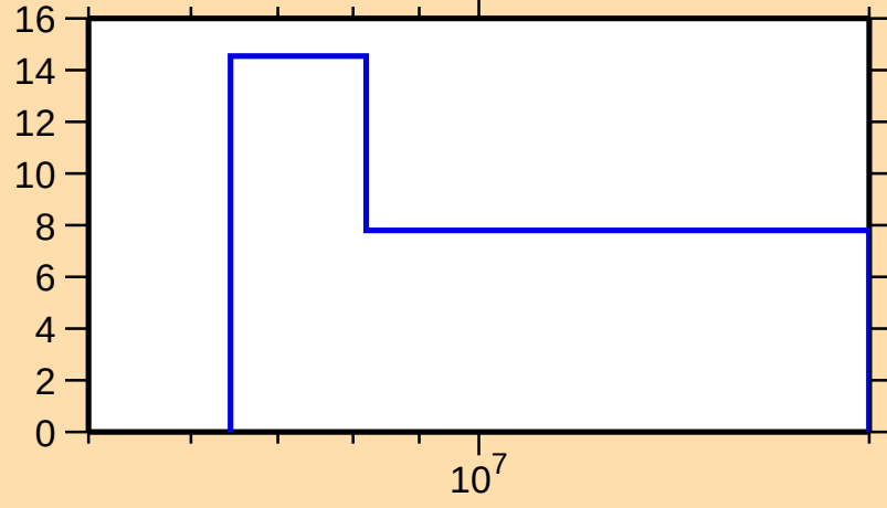
\Delta\sigma/\sigma vs. E for ^{257}\text{Md}(n,\text{tot.})
