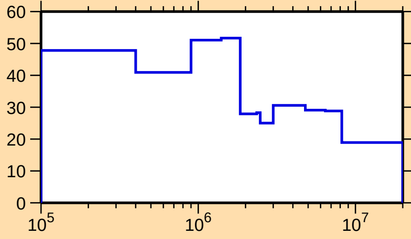
\Delta\sigma/\sigma vs. E for ^{257}\text{Md}(n,\text{el.})
