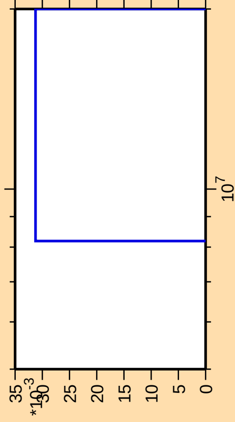
\Delta\sigma/\sigma vs. E for ^{257}\text{Md}(\text{mt } 42)
