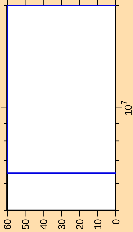
\Delta\sigma/\sigma vs. E for ^{257}\text{Md}(n,n\text{cont.})
