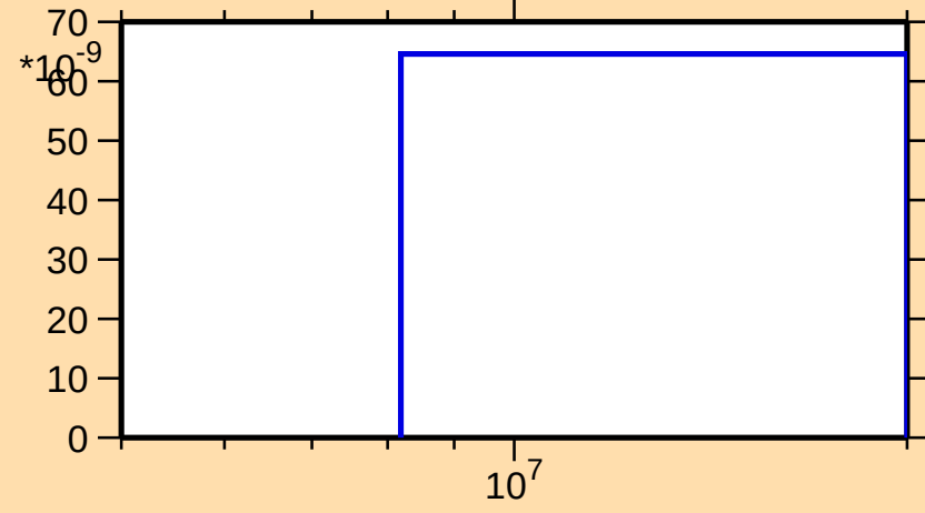
\sigma vs. E for ^{257}\text{Md}(n,\text{nd})
