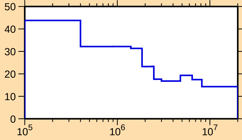
\Delta\sigma/\sigma vs. E for ^{257}\text{Md}(n,\text{nonel.})
