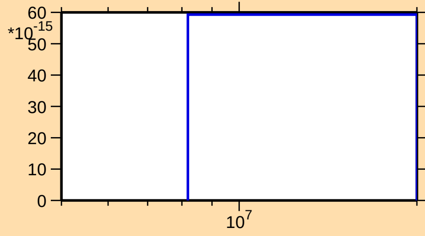
\sigma vs. E for ^{257}\text{Md}(\text{mt } 11)
