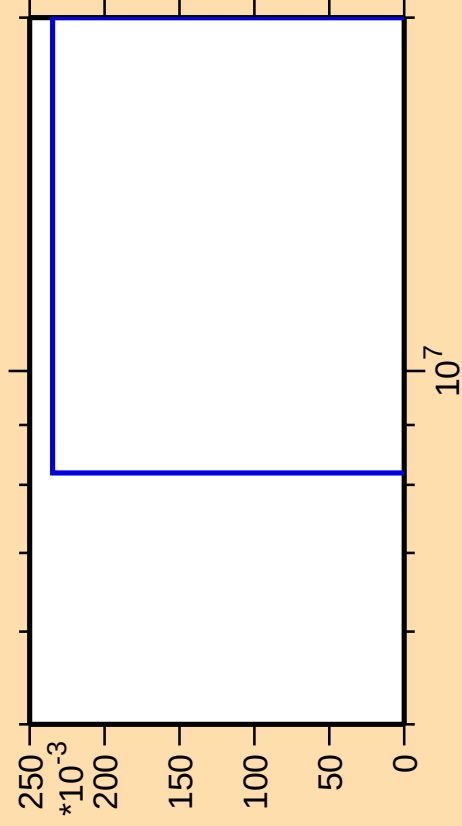
\Delta\sigma/\sigma vs. E for ^{257}\text{Md}(\text{mt } 11)
