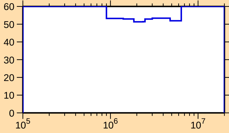
\Delta\sigma/\sigma vs. E for ^{257}\text{Md}(n,n\text{cont.})
