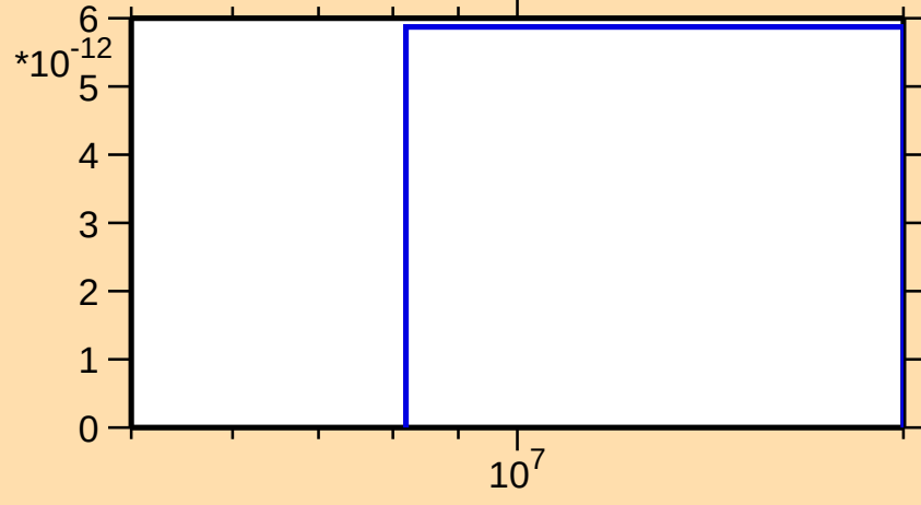
\sigma vs. E for ^{257}\text{Md}(n,\text{He}3)
