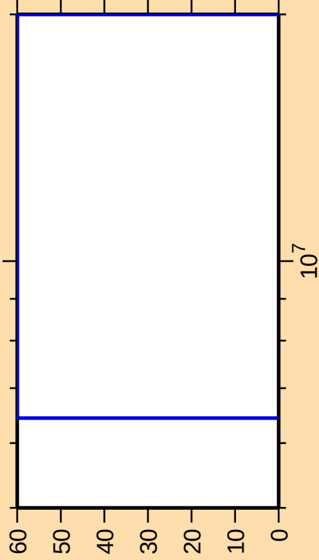
\Delta\sigma/\sigma vs. E for ^{257}\text{Md}(n,n_1)
