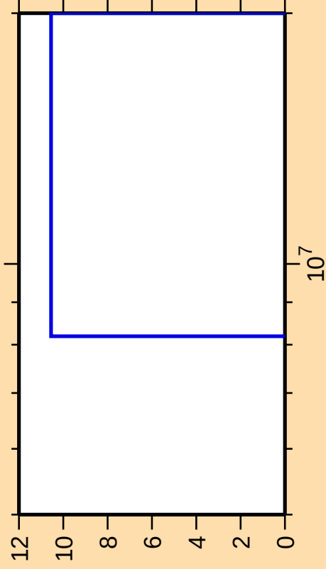
\Delta\sigma/\sigma vs. E for ^{257}\text{Md}(n,\text{He}3)
