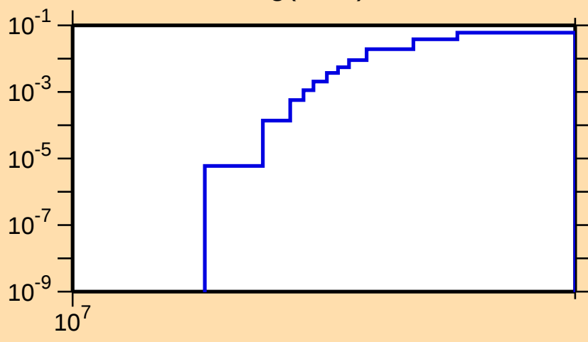
\sigma vs. E for ^{26}\text{Mg}(n,n\alpha)
