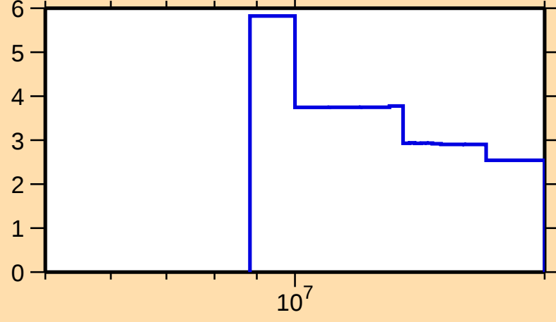
\Delta\sigma/\sigma vs. E for ^{26}\text{Mg}(n,\text{tot.})
