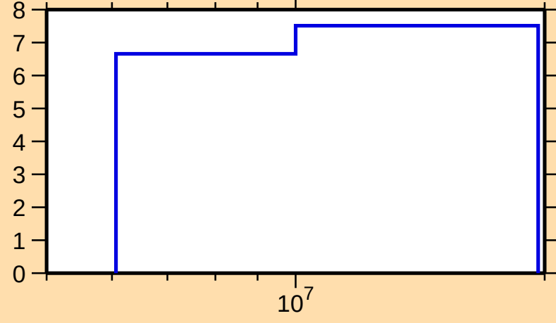
\Delta\sigma/\sigma vs. E for ^{26}\text{Mg}(n,n\text{oncl.})
