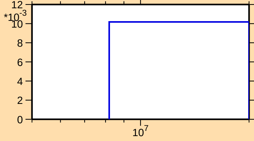
\sigma vs. E for ^{26}\text{Mg}(n,p)
