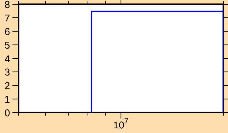
\Delta\sigma/\sigma vs. E for ^{26}\text{Mg}(n,\text{el.})
