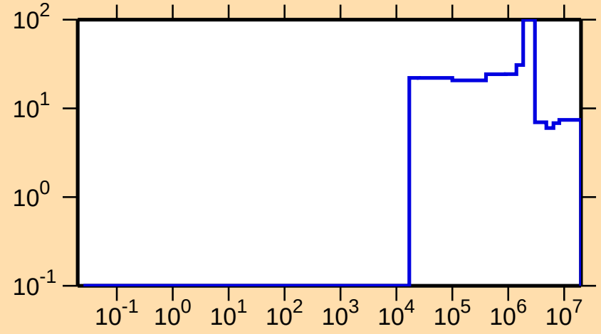
\Delta\sigma/\sigma vs. E for ^{26}\text{Mg}(n,\text{nonel.})
