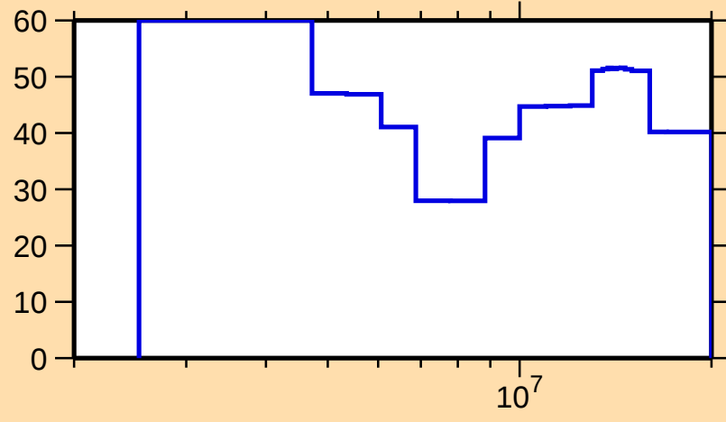
\Delta\sigma/\sigma vs. E for ^{52}\text{Mn}(n,n\text{cont.})
