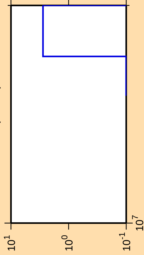
\Delta\sigma/\sigma vs. E for ^{52}\text{Mn}(\text{mt } 45)
