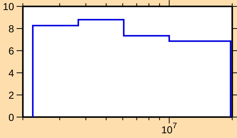
\Delta\sigma/\sigma vs. E for ^{52}\text{Mn}(n,n\text{onel.})
