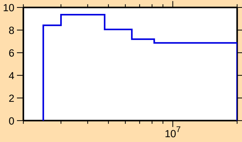
\Delta\sigma/\sigma vs. E for ^{52}\text{Mn}(n,n\text{oncl.})
