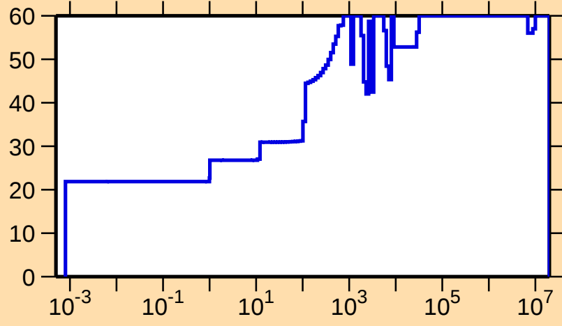
\Delta\sigma/\sigma vs. E for ^{54}\text{Mn}(n,\gamma)
