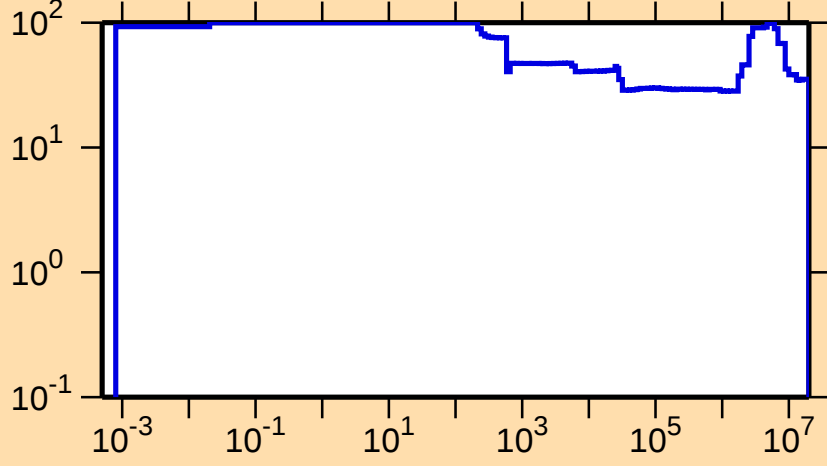
\Delta\sigma/\sigma vs. E for ^{54}\text{Mn}(n,p)
