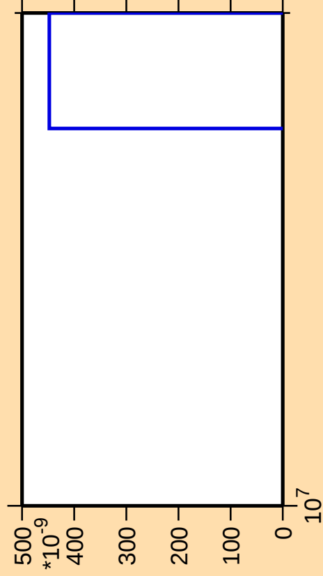
\Delta\sigma/\sigma vs. E for ^{54}\text{Mn}(\text{mt } 34)
