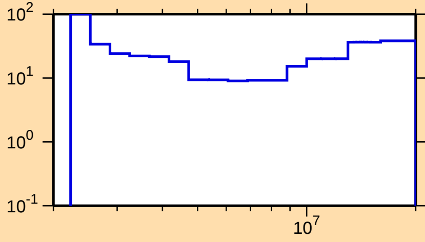
\Delta\sigma/\sigma vs. E for ^{54}\text{Mn}(n,n\text{cont.})
