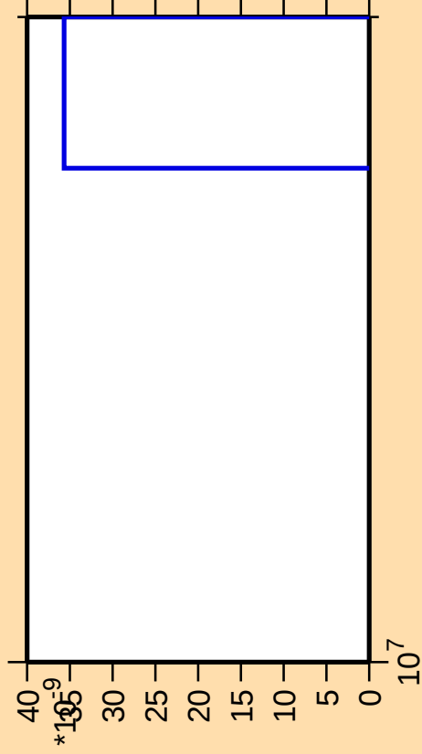
\Delta\sigma/\sigma vs. E for ^{54}\text{Mn}(n,\text{nt})
