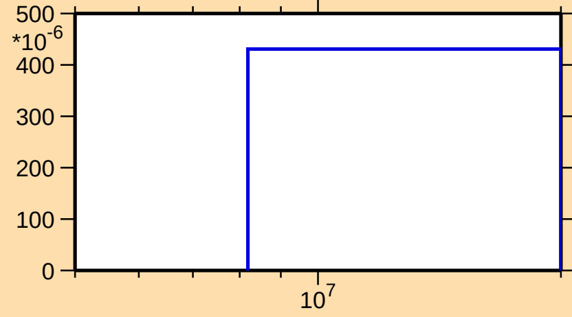
\sigma vs. E for ^{54}\text{Mn}(n,n\alpha)
