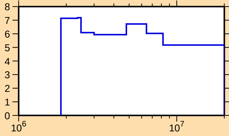
\Delta\sigma/\sigma vs. E for ^{54}\text{Mn}(n,n\text{onel.})
