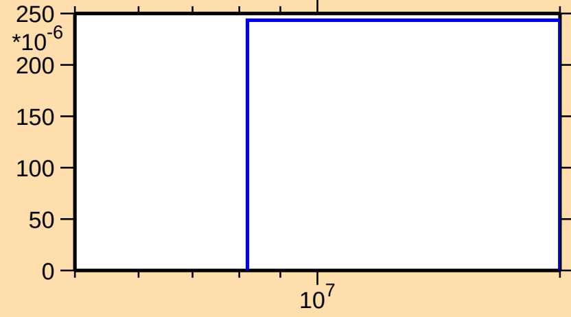
\sigma vs. E for ^{54}\text{Mn}(n,p\alpha)
