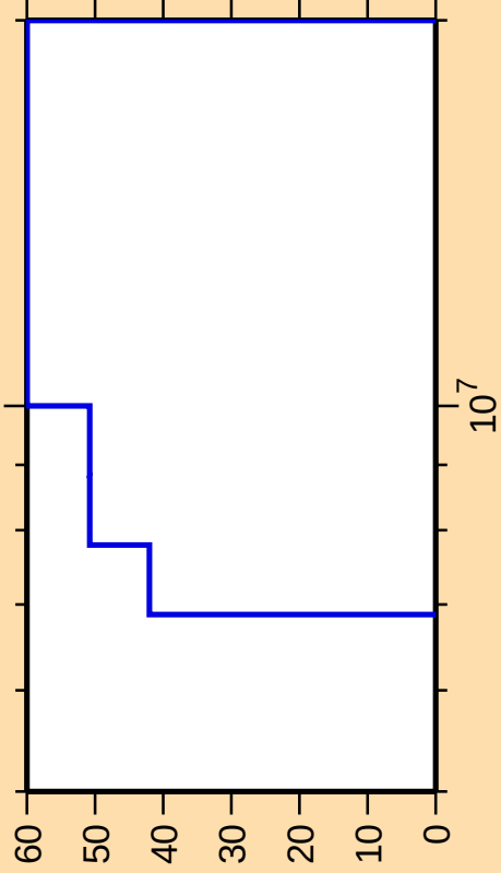
\Delta\sigma/\sigma vs. E for ^{56}\text{Mn}(n,n\text{cont.})
