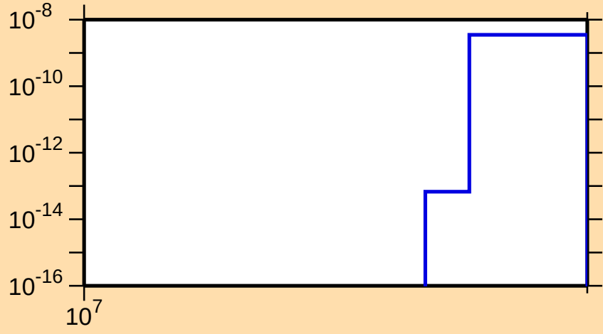
\sigma vs. E for ^{56}\text{Mn}(n,\text{He3})
