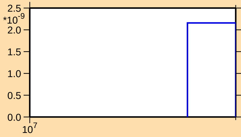
\sigma vs. E for ^{56}\text{Mn}(n,2n\alpha)
