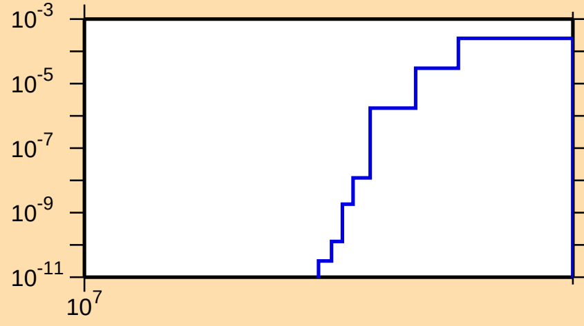
\sigma vs. E for ^{56}\text{Mn}(n,\text{nd})
