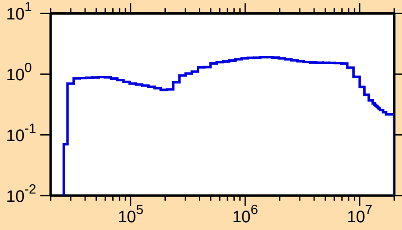
\sigma vs. E for ^{56}\text{Mn}(n,\text{inel.})
