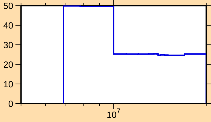
\Delta\sigma/\sigma vs. E for ^{56}\text{Mn}(n,2n)
