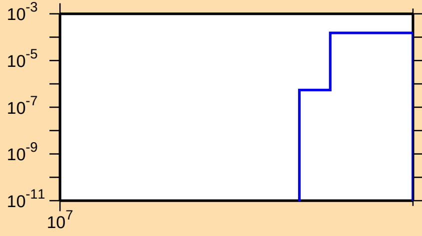
\sigma vs. E for ^{56}\text{Mn}(n,2np)
