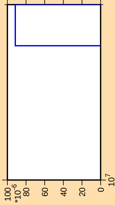
\Delta\sigma/\sigma vs. E for ^{56}\text{Mn}(\text{mt117})
