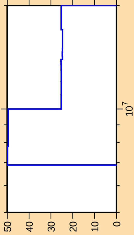
\Delta\sigma/\sigma vs. E for ^{56}\text{Mn}(n,2n)
