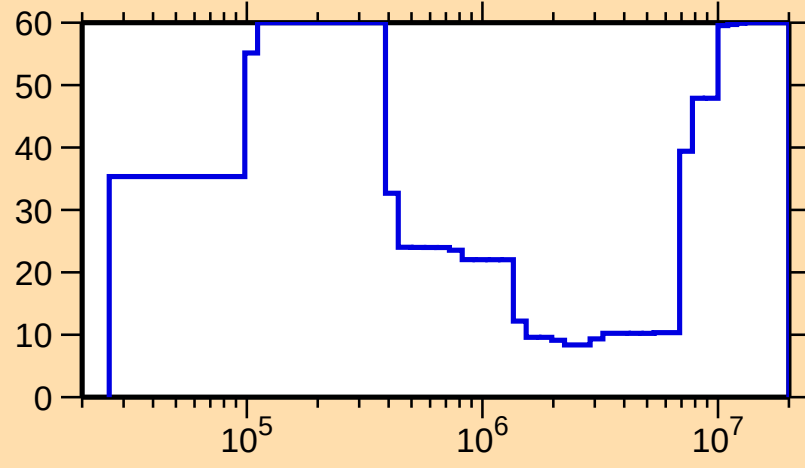
\Delta\sigma/\sigma vs. E for ^{56}\text{Mn}(n,\text{inel.})
