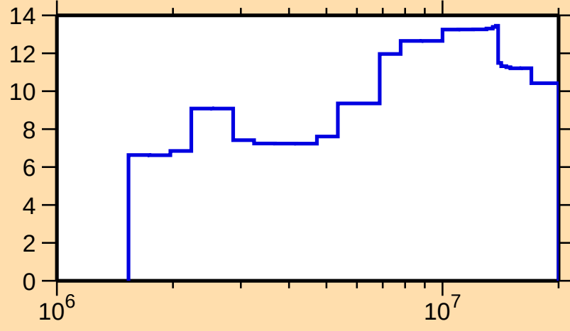
\Delta\sigma/\sigma vs. E for ^{56}\text{Mn}(n,\text{el.})
