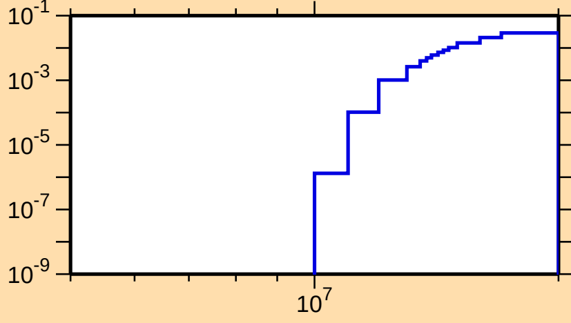
\sigma vs. E for ^{56}\text{Mn}(n,np)
