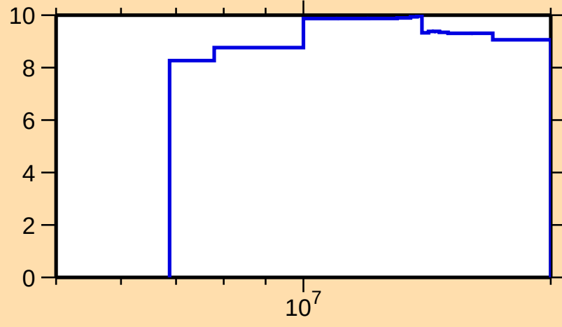
\Delta\sigma/\sigma vs. E for ^{56}\text{Mn}(n,\text{tot.})
