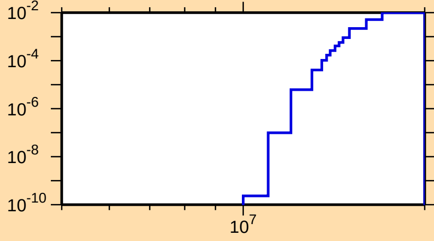
\sigma vs. E for ^{56}\text{Mn}(n,n\alpha)
