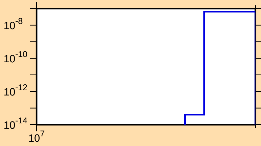
\sigma vs. E for ^{56}\text{Mn}(n,nt)
