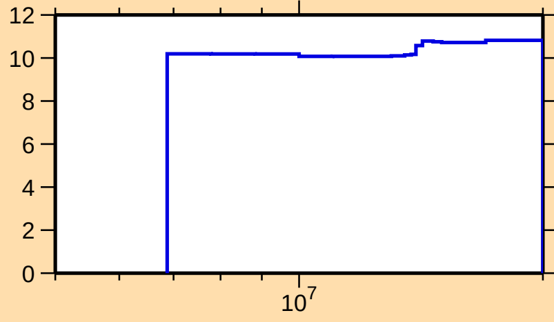
\Delta\sigma/\sigma vs. E for ^{56}\text{Mn}(n,\text{nonel.})
