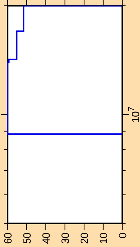
\Delta\sigma/\sigma vs. E for ^{56}\text{Mn}(n,np)
