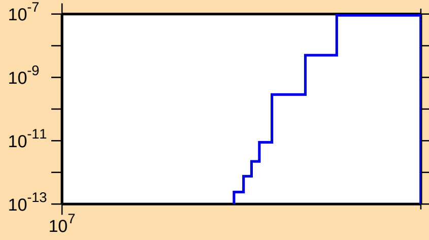
\sigma vs. E for ^{56}\text{Mn}(n,p\alpha)
