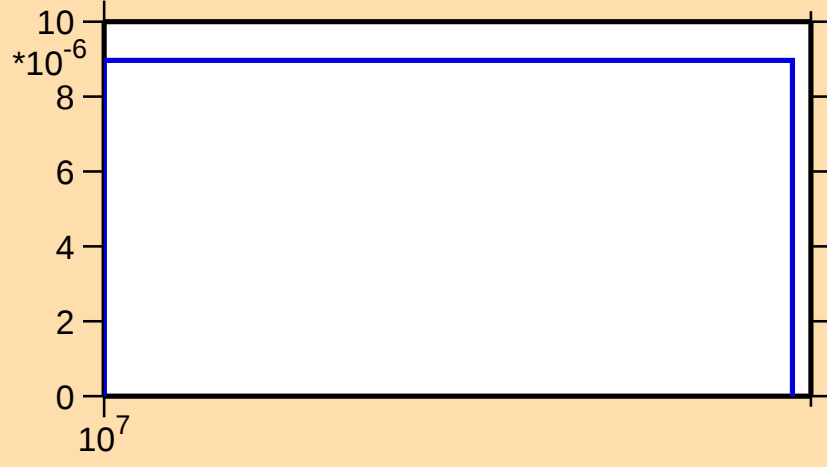
\sigma vs. E for ^{56}\text{Mn}(n,3n)
