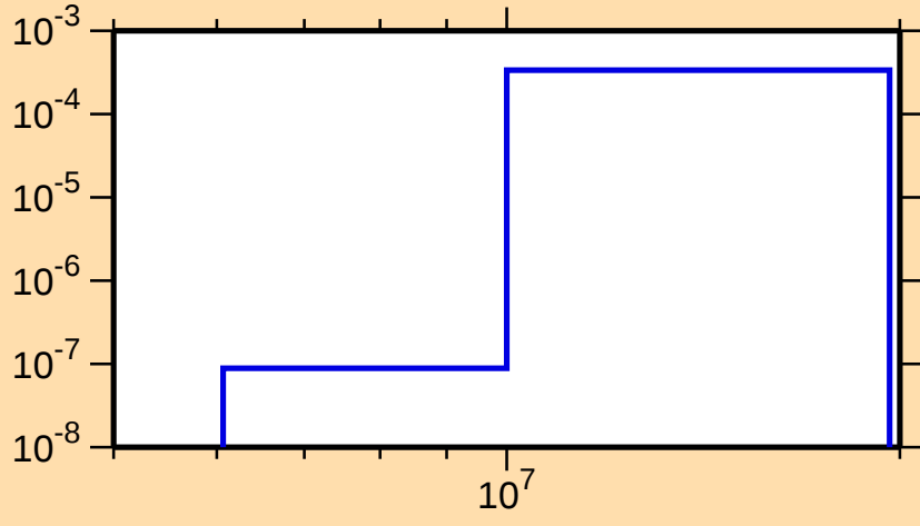
\sigma vs. E for ^{56}\text{Mn}(n,t)
