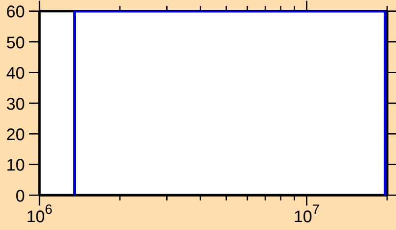
\Delta\sigma/\sigma vs. E for ^{56}\text{Mn}(n,\gamma)
