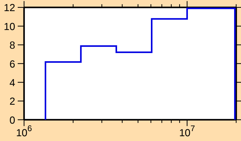
\Delta\sigma/\sigma vs. E for ^{56}\text{Mn}(n,\text{el.})
