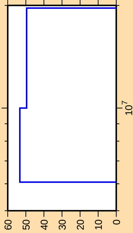
\Delta\sigma/\sigma vs. E for ^{56}\text{Mn}(n,n_1)
