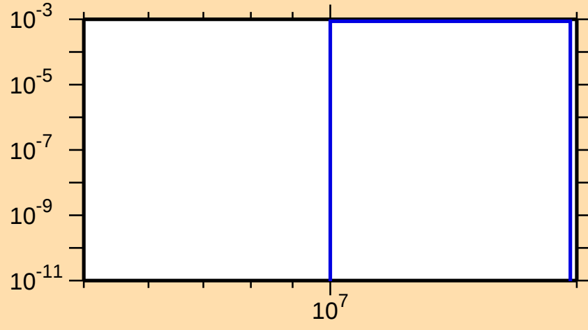
\sigma vs. E for ^{56}\text{Mn}(n,n\alpha)
