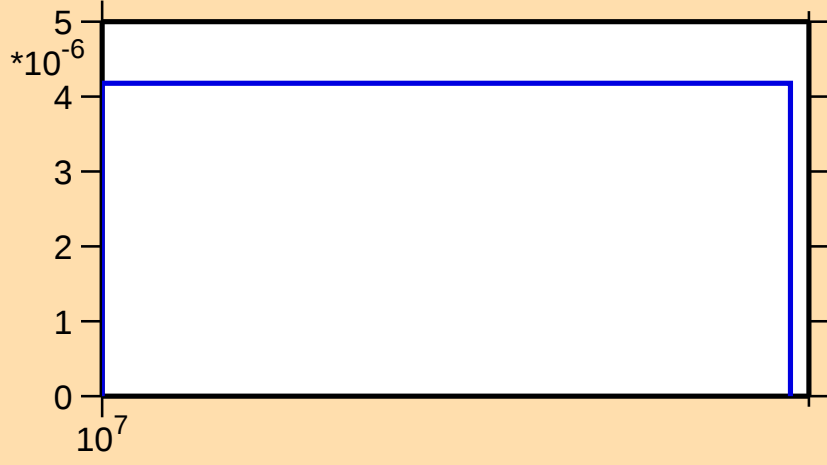
\sigma vs. E for ^{56}\text{Mn}(n,\text{nd})
